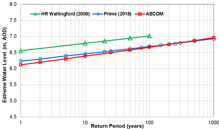
Figure A-1: Comparison of extreme sea level estimates
