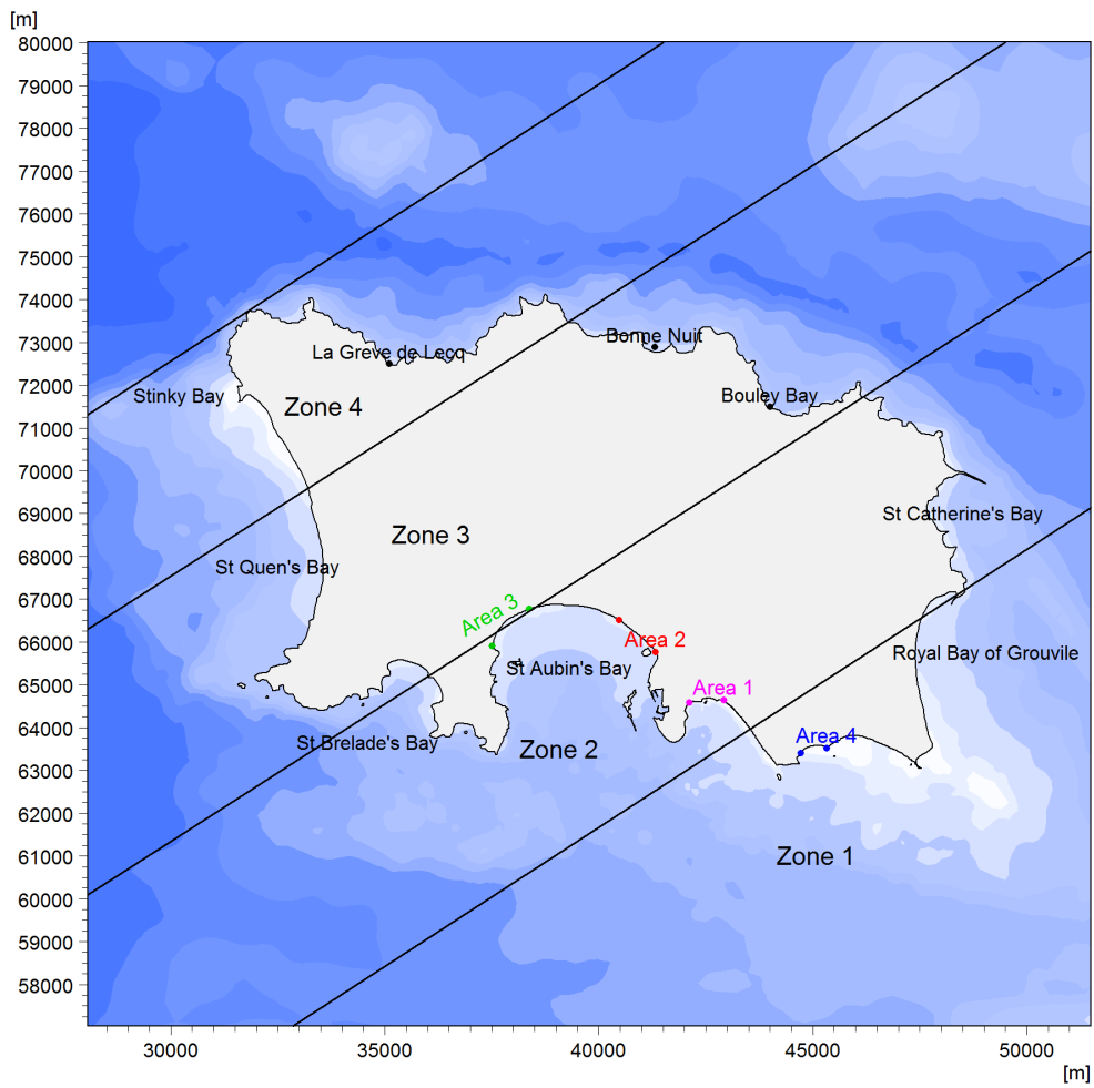
Figure A-3: Zones defined for extreme sea level adjustments
