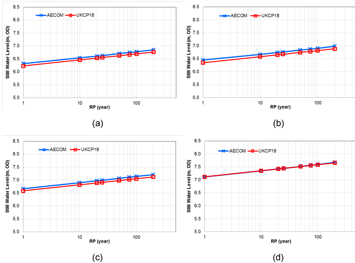
Figure A-6: Comparison of extreme water level between AECOM and UKCP18 (a) 2020 (b) 2040 (c) 2070 and (d) 2100
