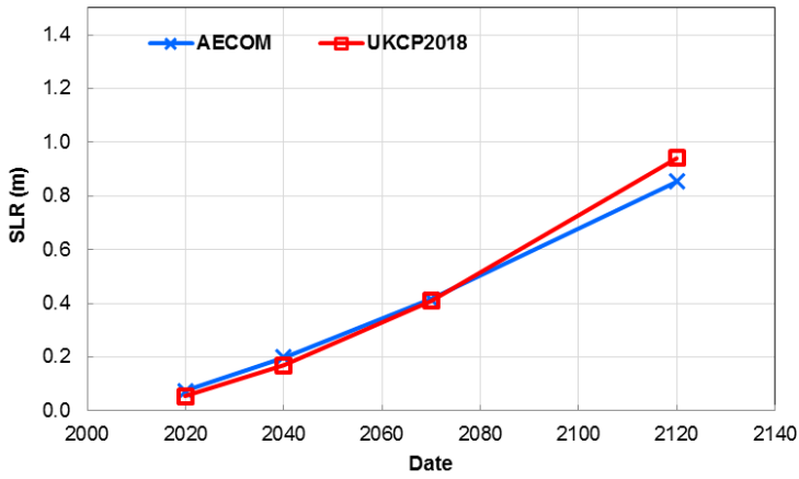
Figure A-5: Comparison of SLR AECOM and UKCP18
