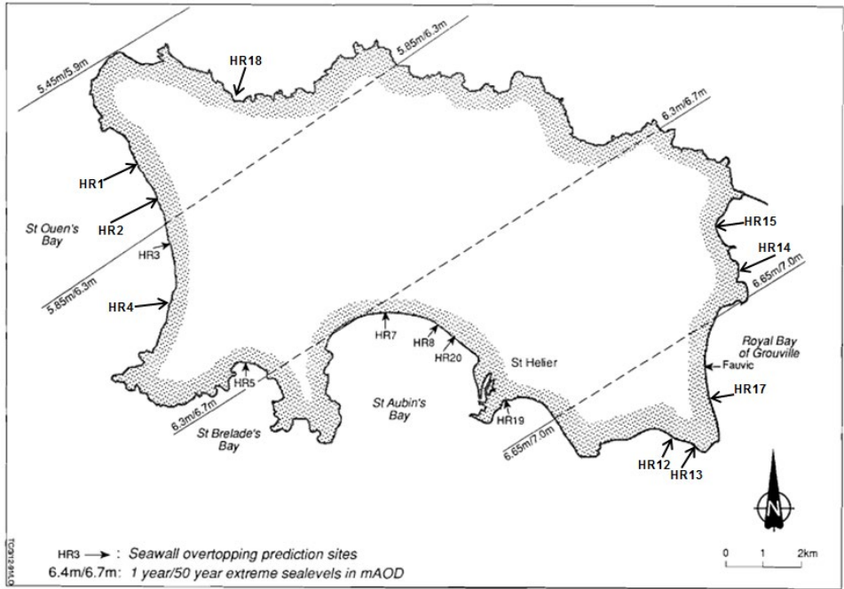
Figure A-2: Location of extreme sea level estimates (HR Wallingford, 1991)
