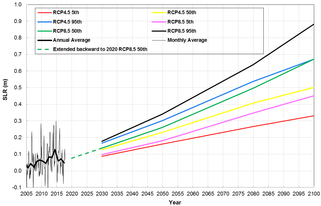
Figure A-4: Historic mean sea level variation and SLR under RCP4.5 and RCP8.5 climate change scenarios
