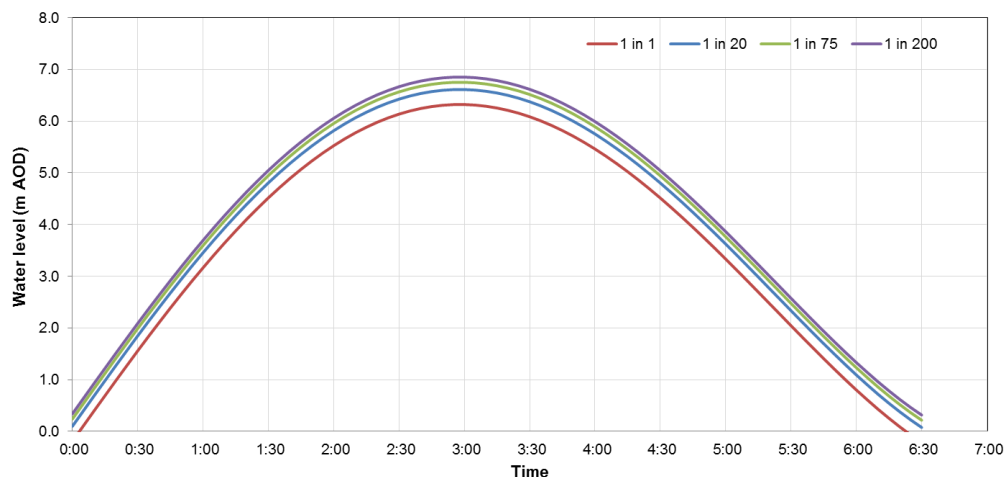
Figure G-29: Water Level Profiles (2020)
