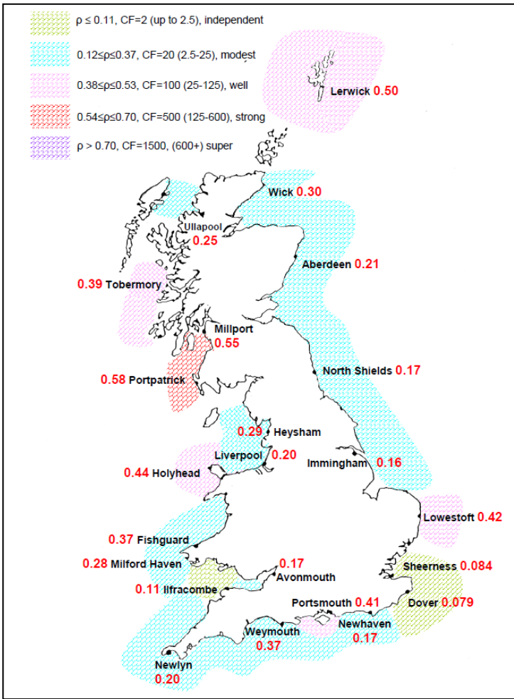
Figure G-2: Correlation coefficient (p, wave height & sea level): all wave directions
