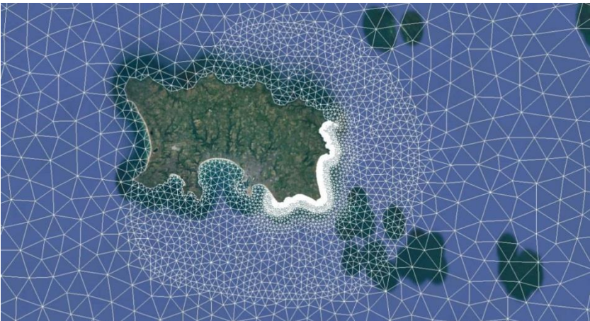
Figure G-16: View of Enhanced Nearshore Mesh Resolution along the East Coast (Model D)
