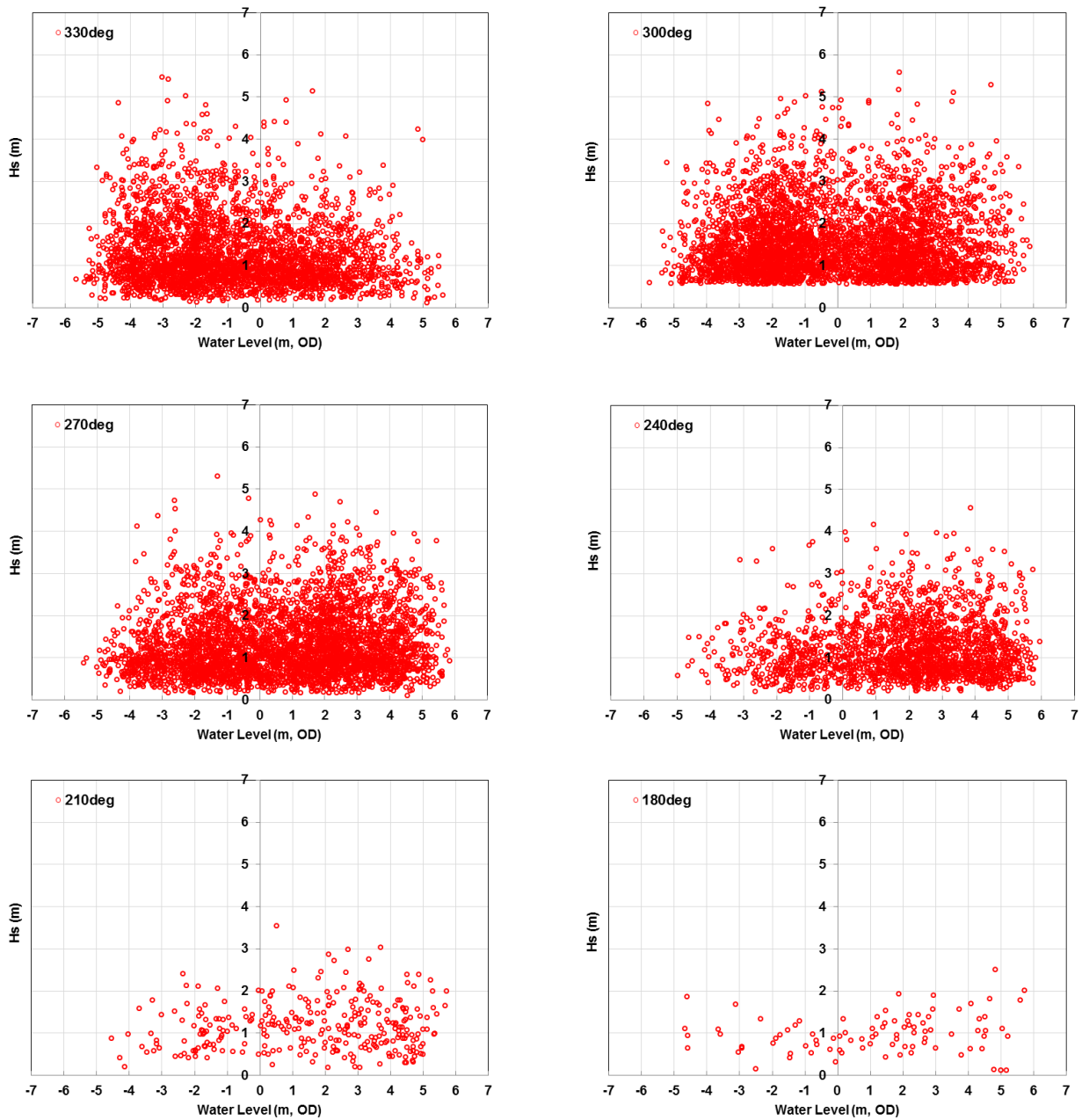
Figure G-5: Directional Scatter Plot of Wave Height against Water Level
