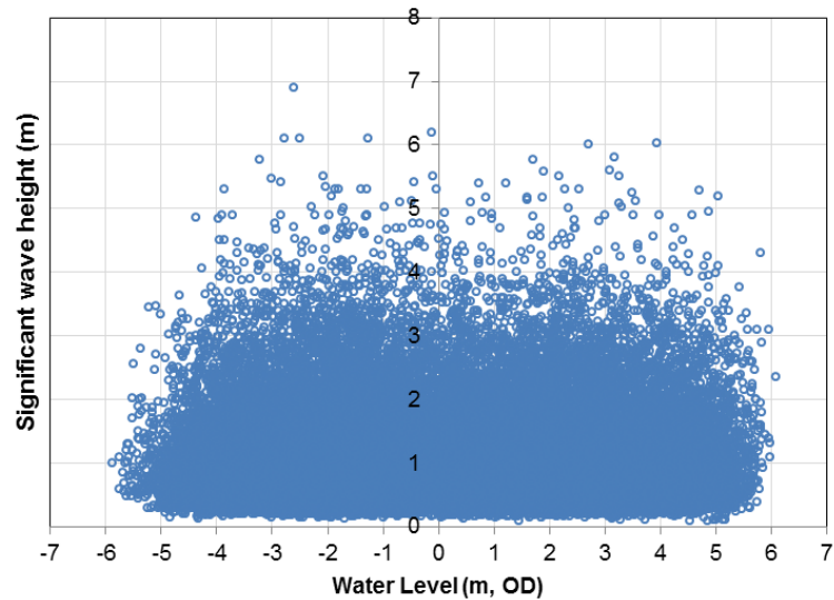
Figure G-4: Plot of Wave Height against Water Level
