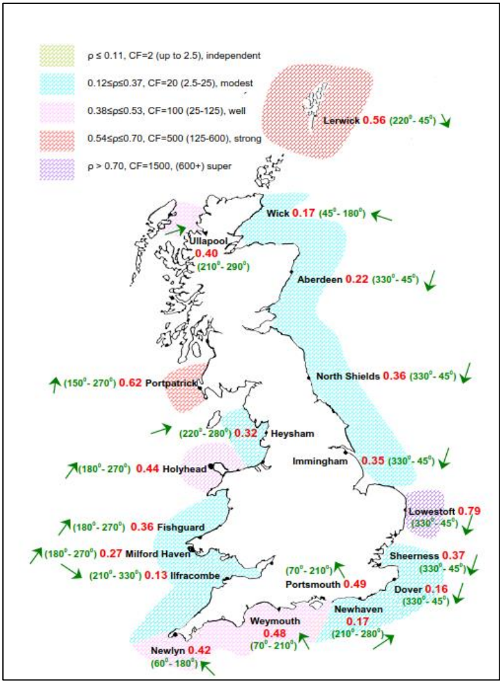
Figure G-3. Correlation Coefficient ( p , Wave Height & Sea Level): Wave Direction where Dependence is Highest
