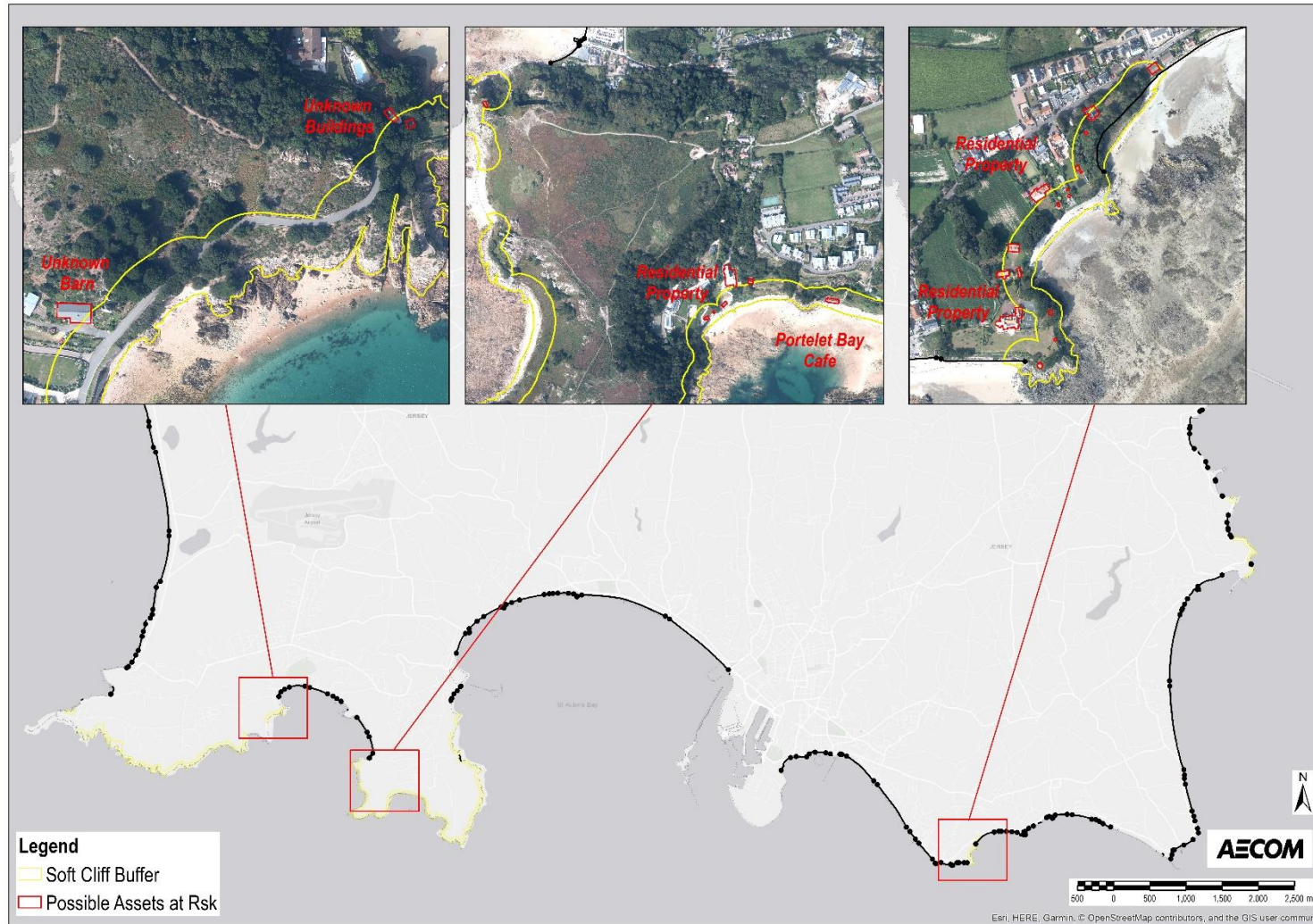
Figure I-5: Assets present in future buffer zone – Les Creux, Le Ouaisné and Portelet Beach, and St Clement (between Green Island defences and Le Nez Point to Le Hocq Point defences)
