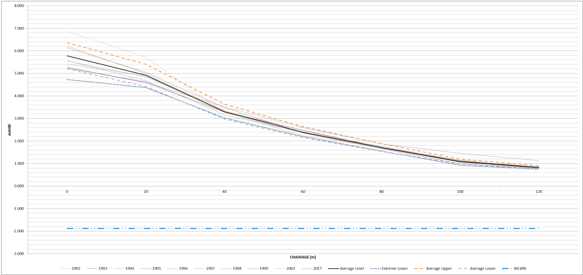
Figure I-41: Annual change of historic beach profiles, compared with extreme averages – PSD3
