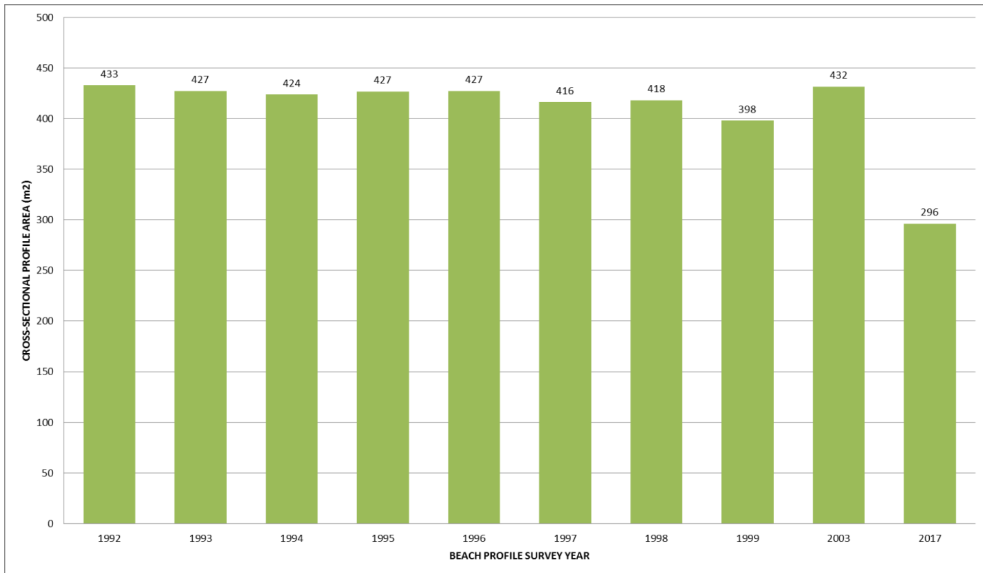
Figure I-76: Cross sectional Area of Annual Average Profiles – HR18
