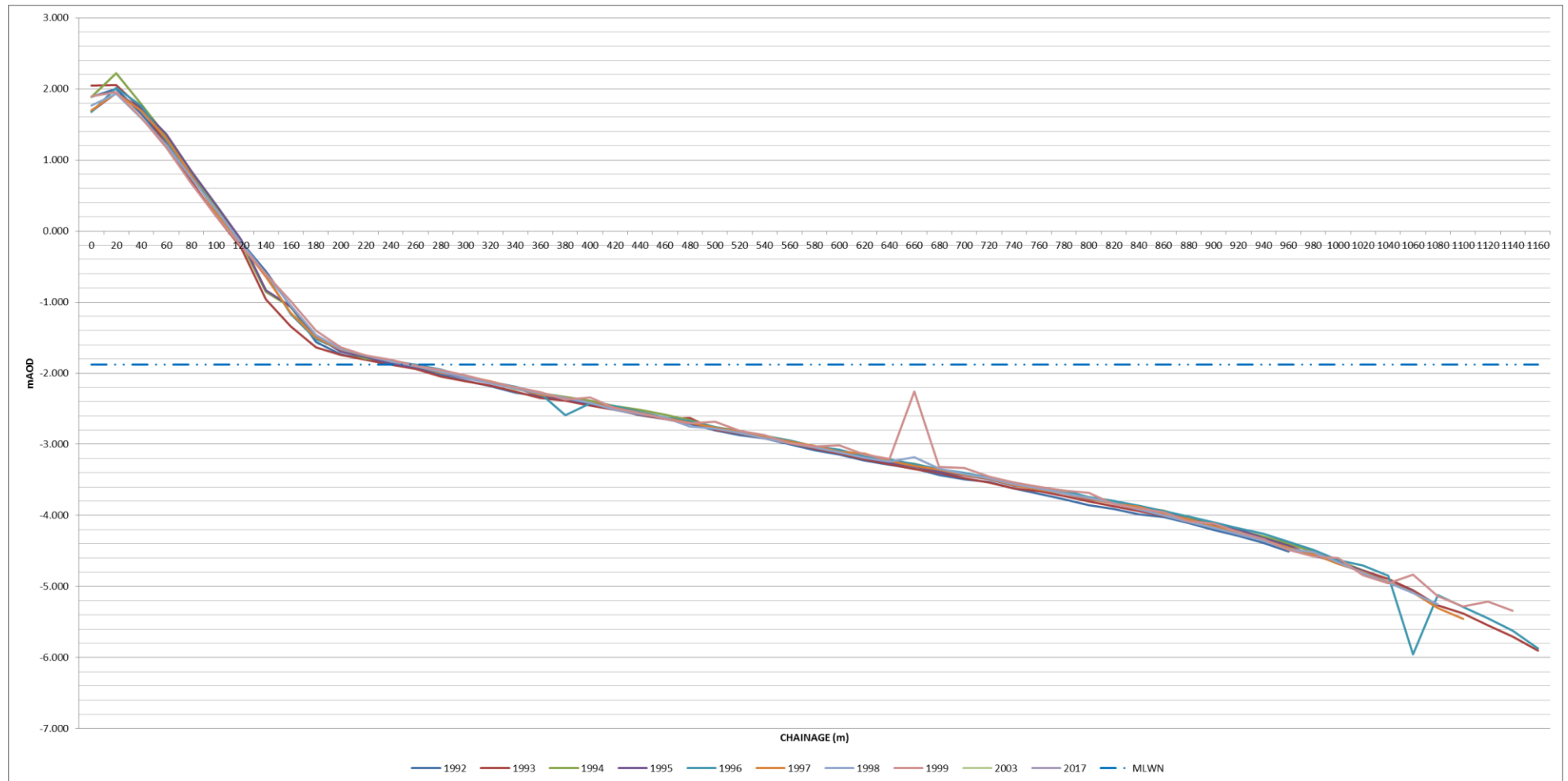
Figure I-31: Annual change of historic beach profiles – HR15
