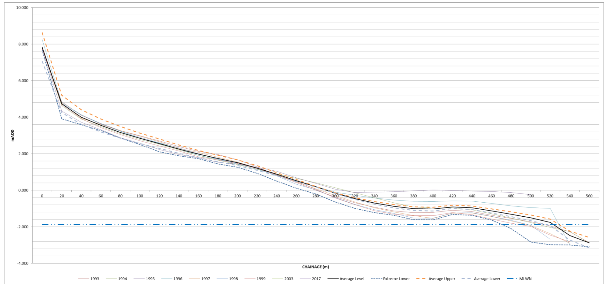
Figure I-54: Annual change of historic beach profiles, compared with extreme averages – HR7
