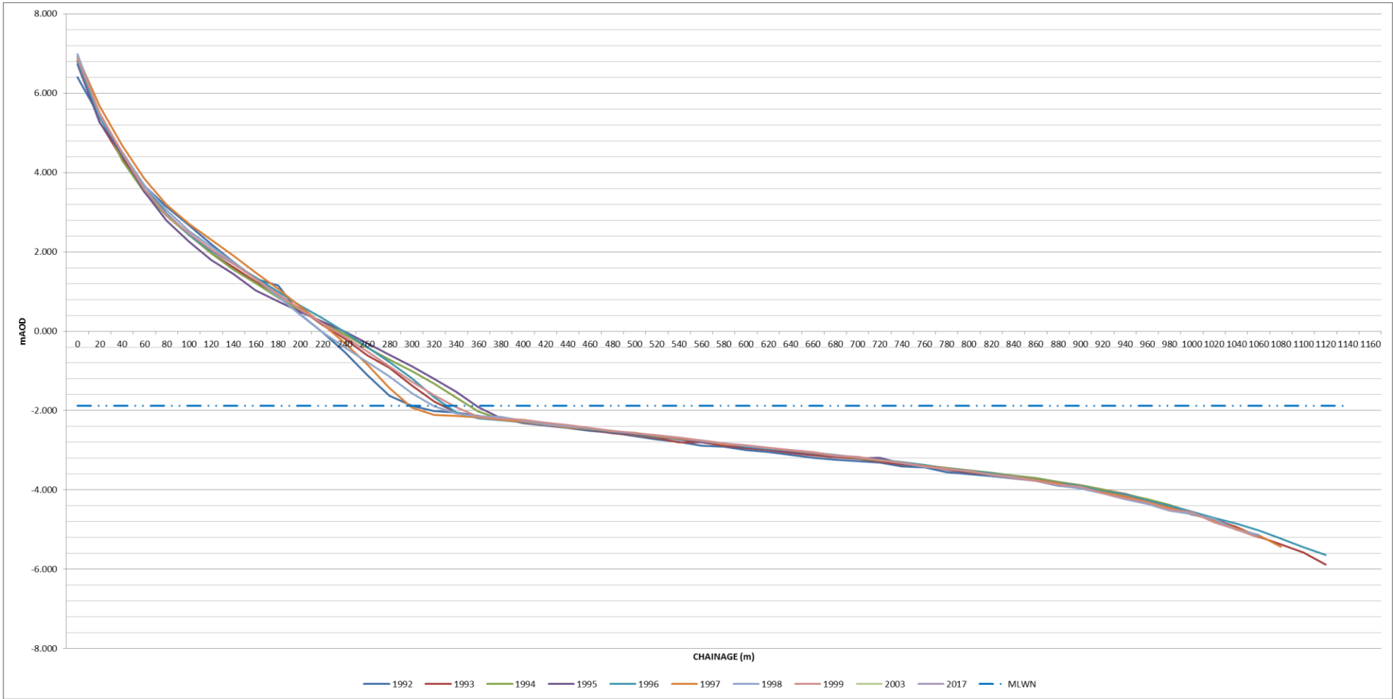
Figure I-30: Annual change of historic beach profiles – HR14
