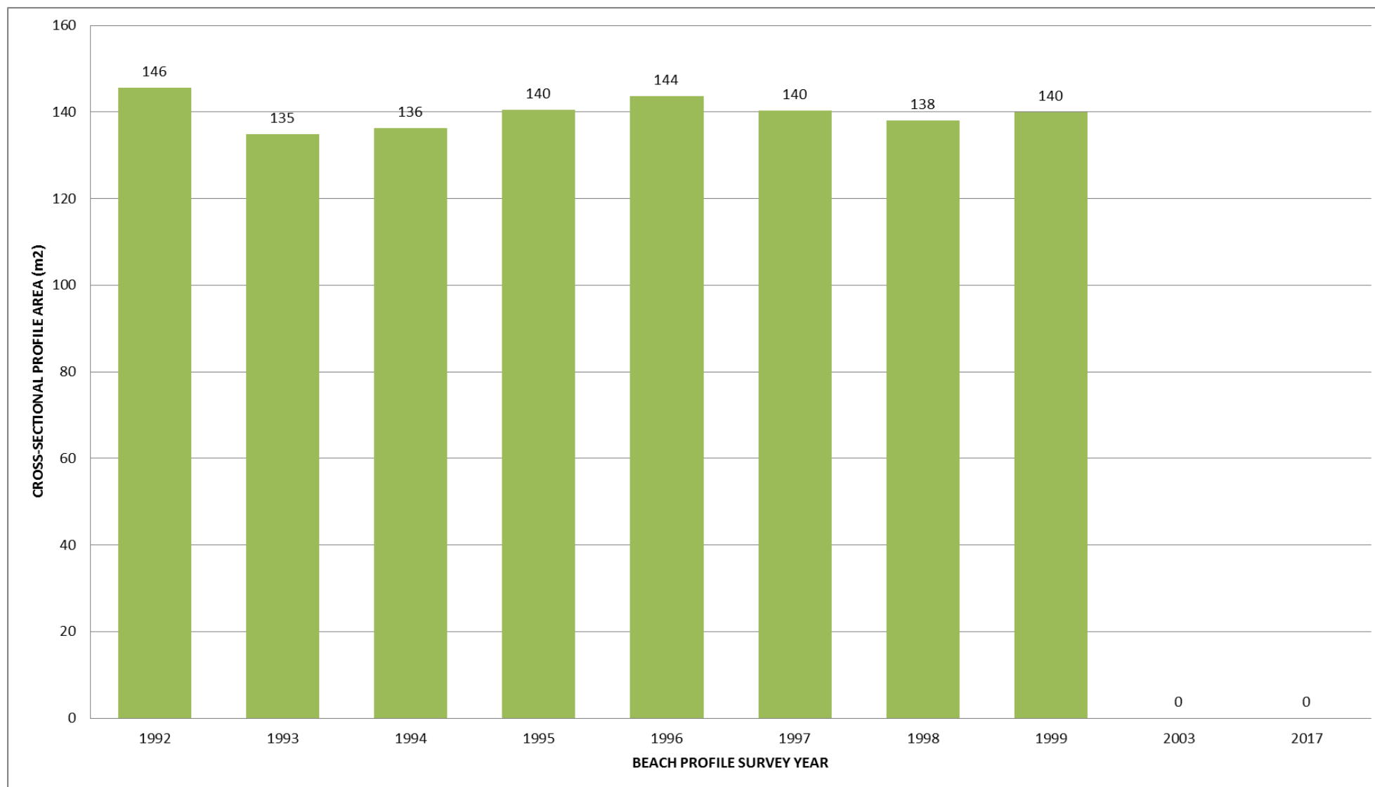
Figure I-70: Cross sectional Area of Annual Average Profiles – PSD4
