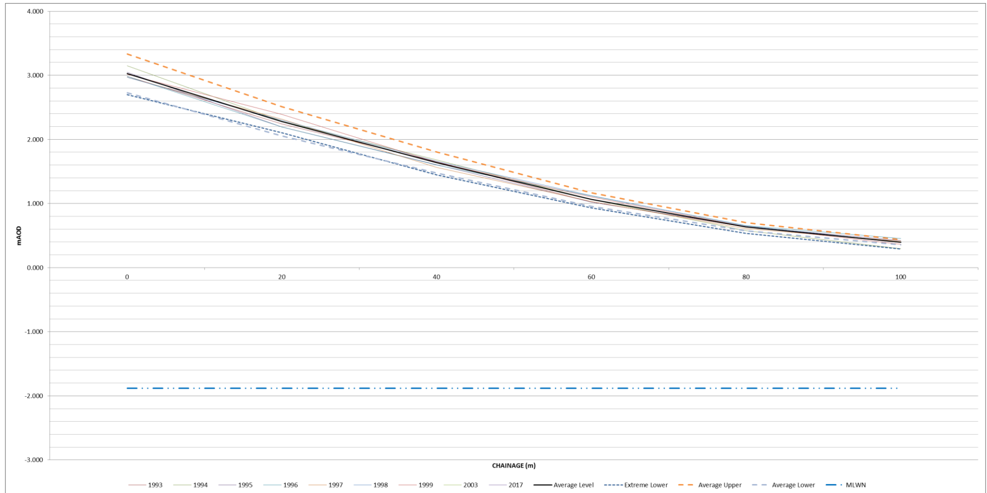
Figure I-43: Annual change of historic beach profiles, compared with extreme averages – PSD5
