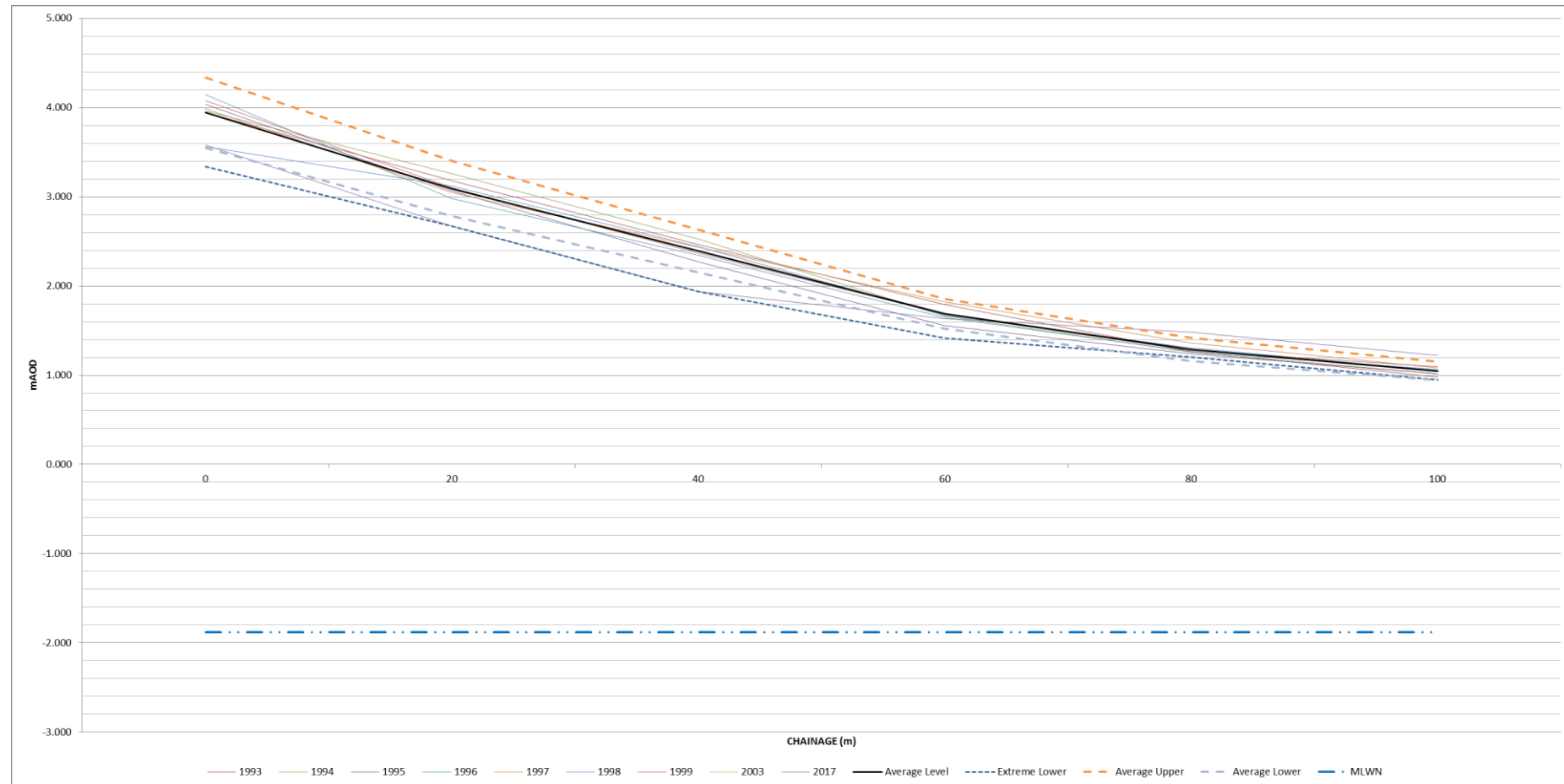
Figure I-39: Annual change of historic beach profiles, compared with extreme averages – PSD1
