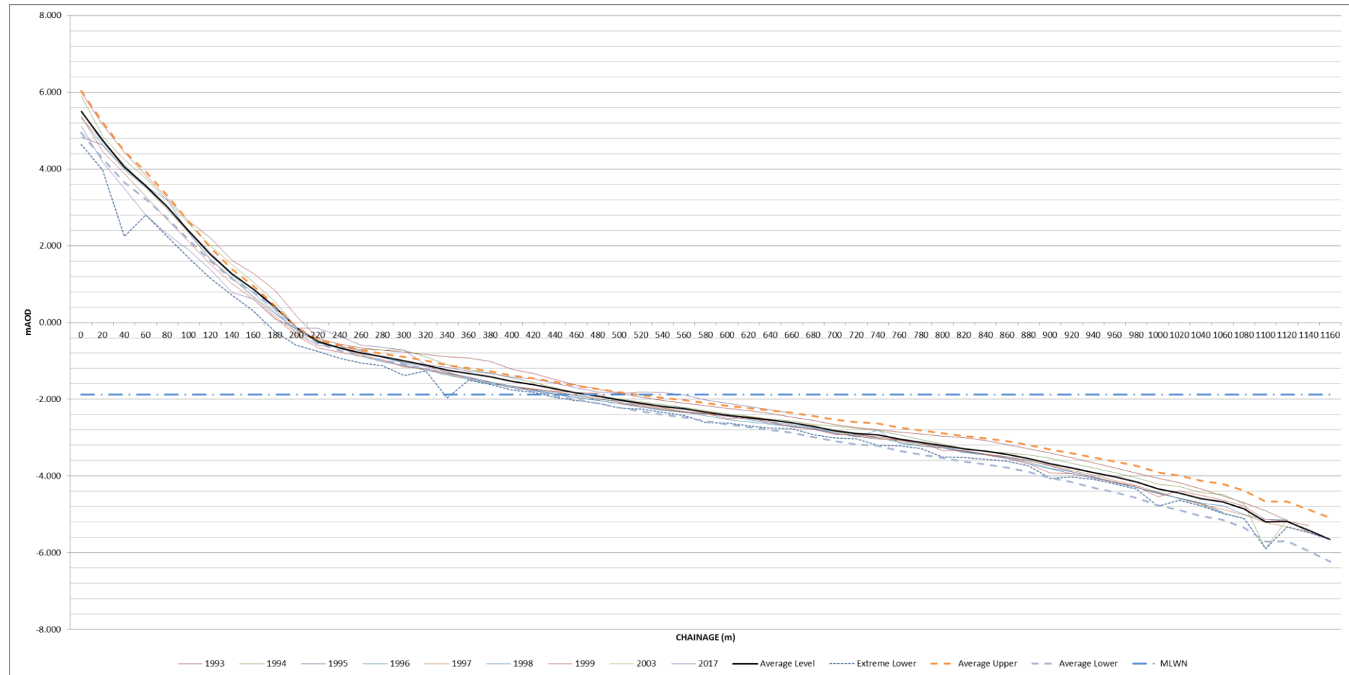
Figure I-59: Annual change of historic beach profiles, compared with extreme averages – HR12
