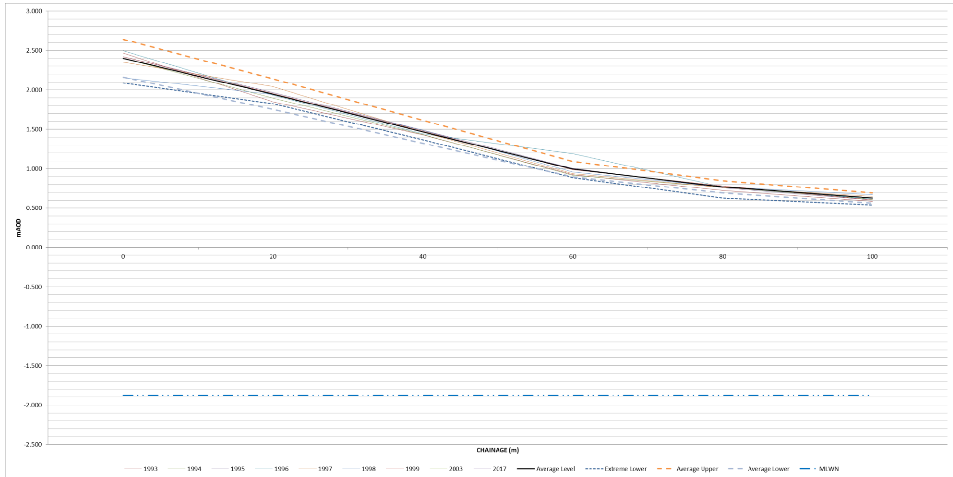
Figure I-42: Annual change of historic beach profiles, compared with extreme averages – PSD4
