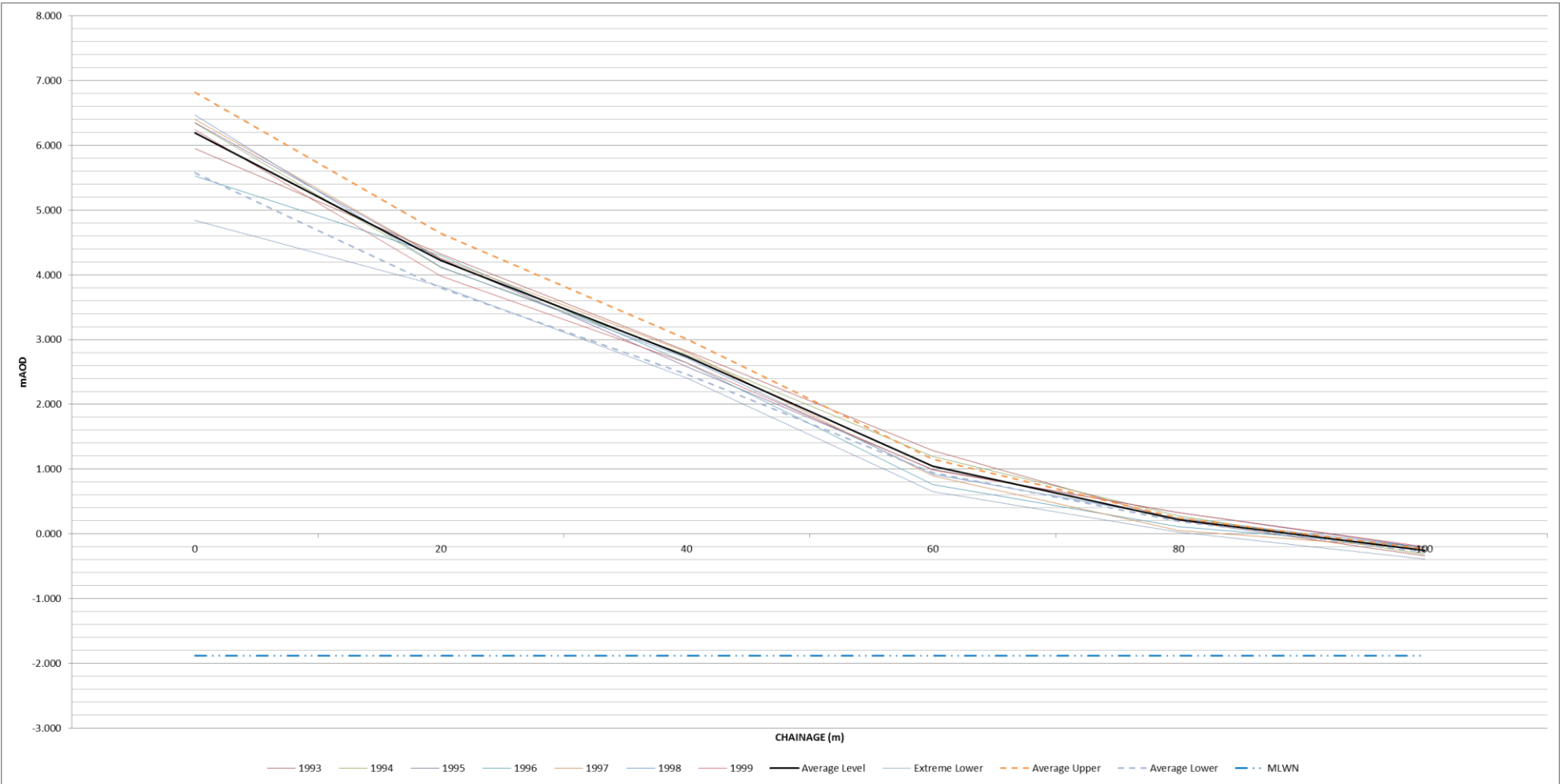
Figure I-46: Annual change of historic beach profiles, compared with extreme averages – PSD8
