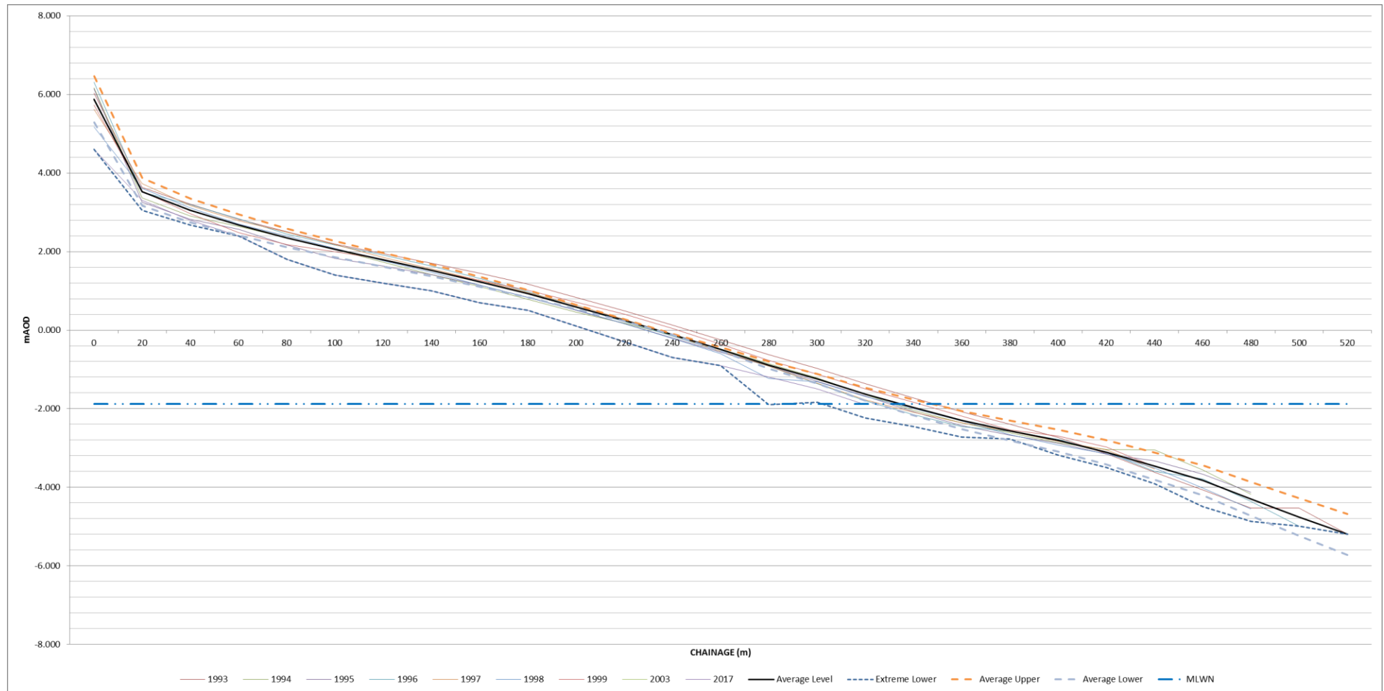
Figure I-53: Annual change of historic beach profiles, compared with extreme averages – HR6
