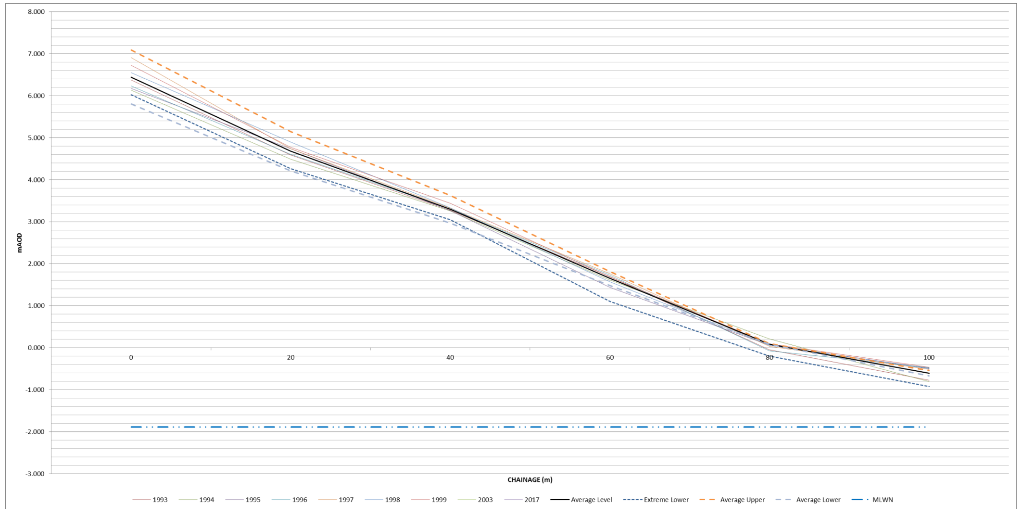
Figure I-47: Annual change of historic beach profiles, compared with extreme averages – PSD9
