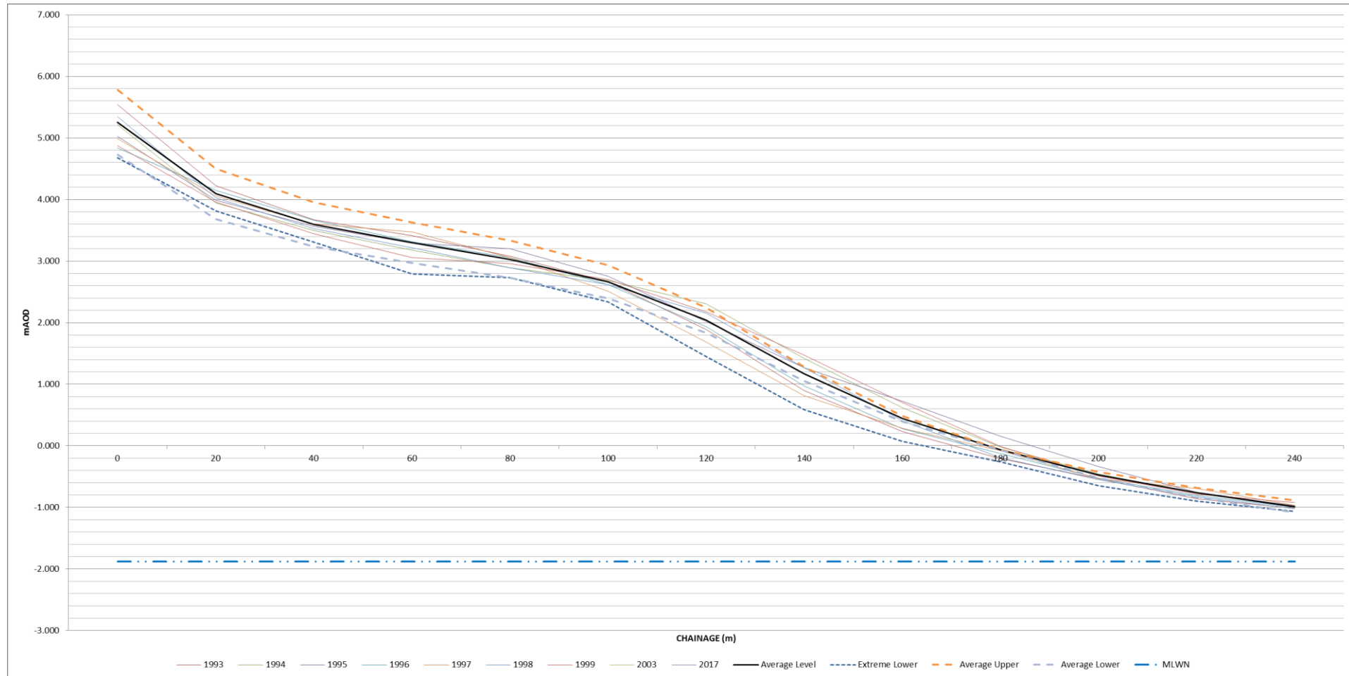
Figure I-48: Annual change of historic beach profiles, compared with extreme averages – HR1
