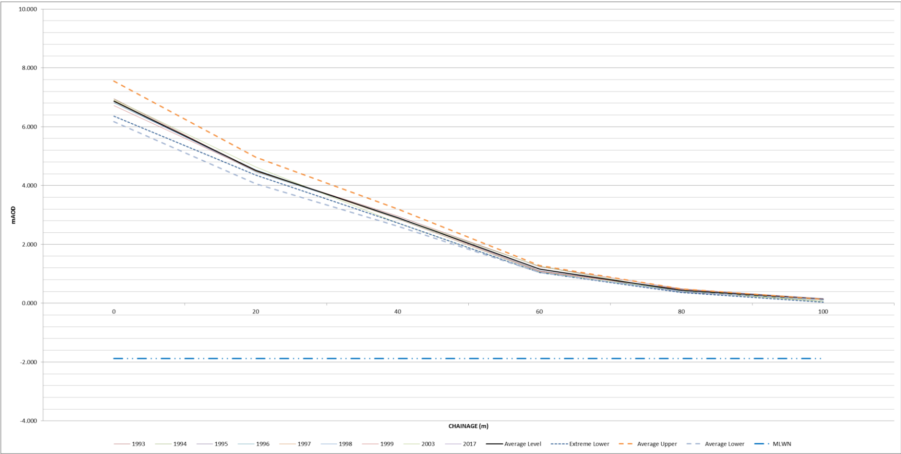
Figure I-69: Annual change of historic beach profiles, compared with extreme averages – HR22
