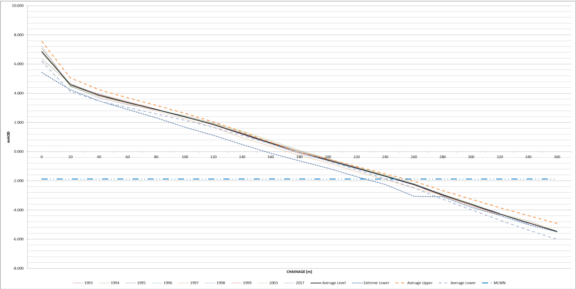
Figure I-58: Annual change of historic beach profiles, compared with extreme averages – HR11
