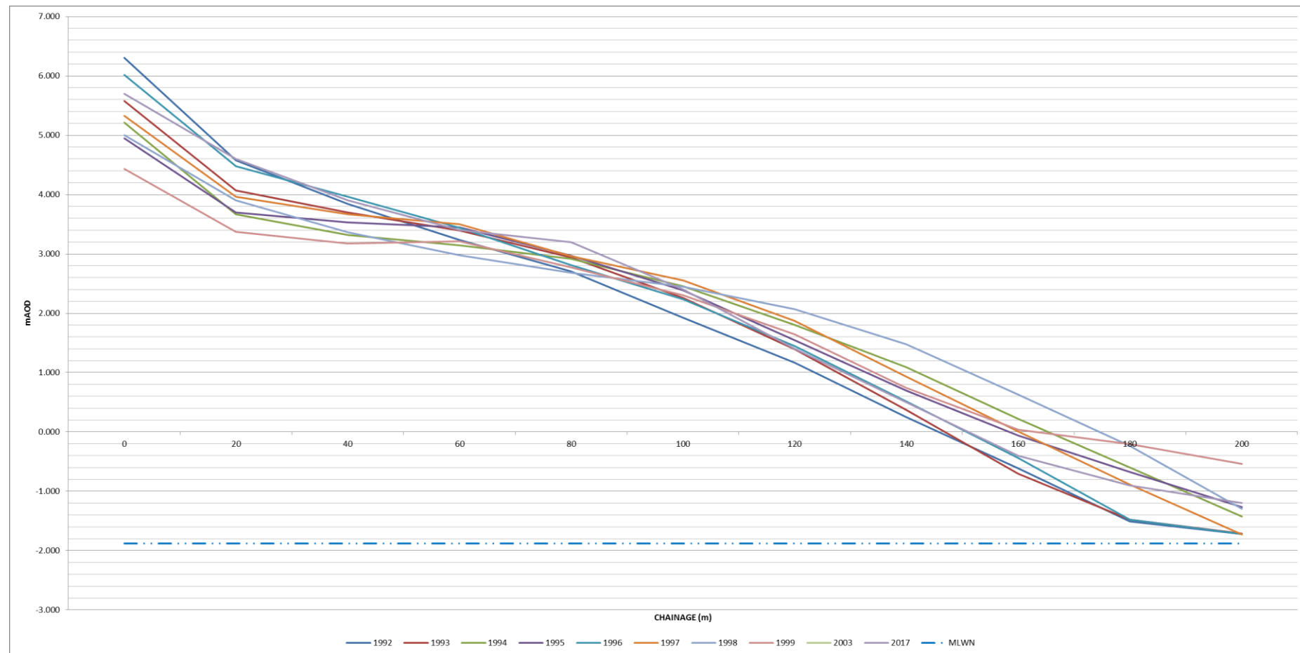
Figure I-18: Annual change of historic beach profiles – HR2
