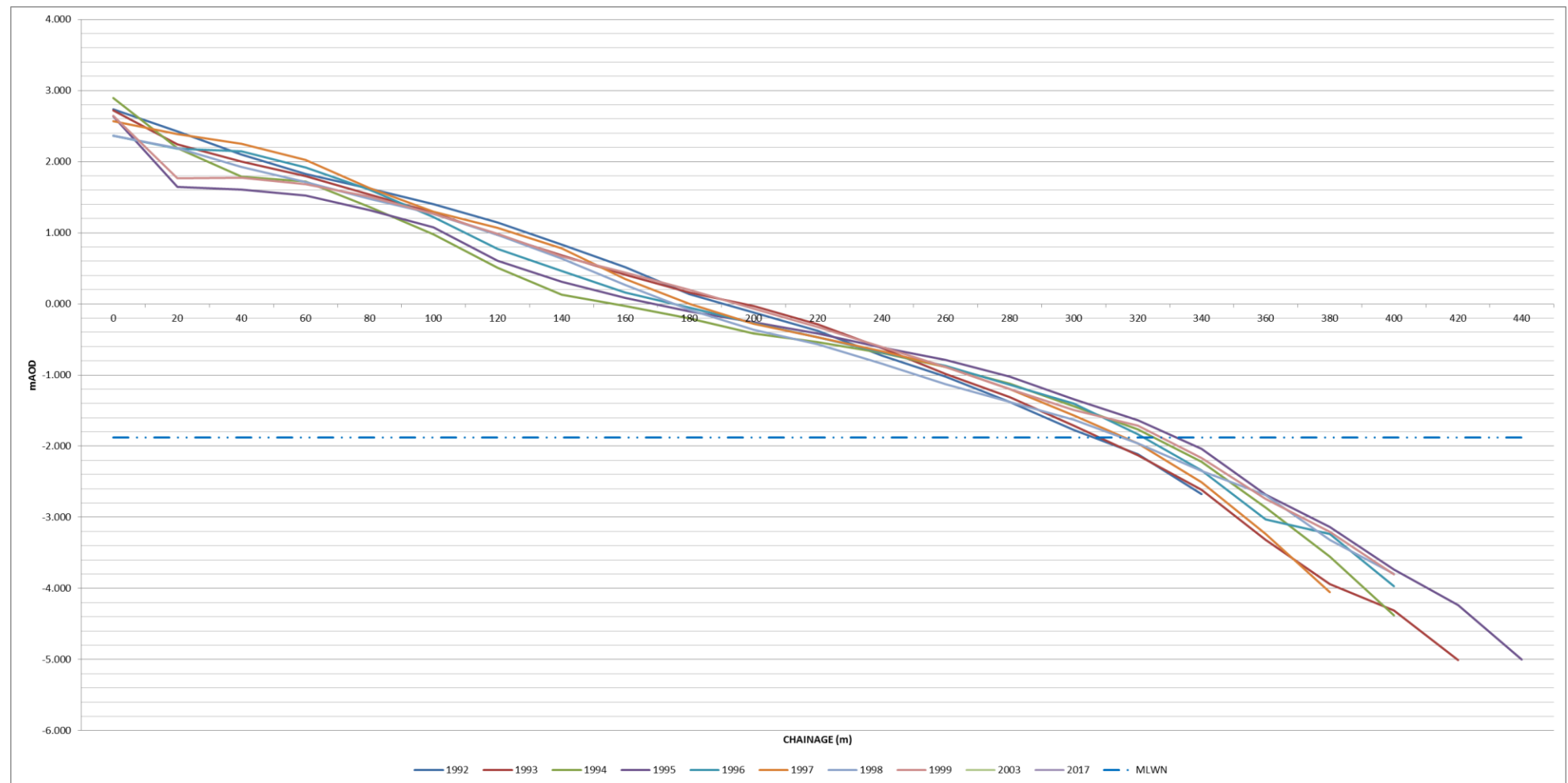
Figure I-20: Annual change of historic beach profiles – HR4
