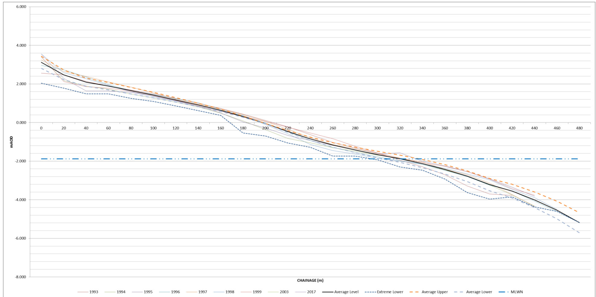
Figure I-52: Annual change of historic beach profiles, compared with extreme averages – HR5
