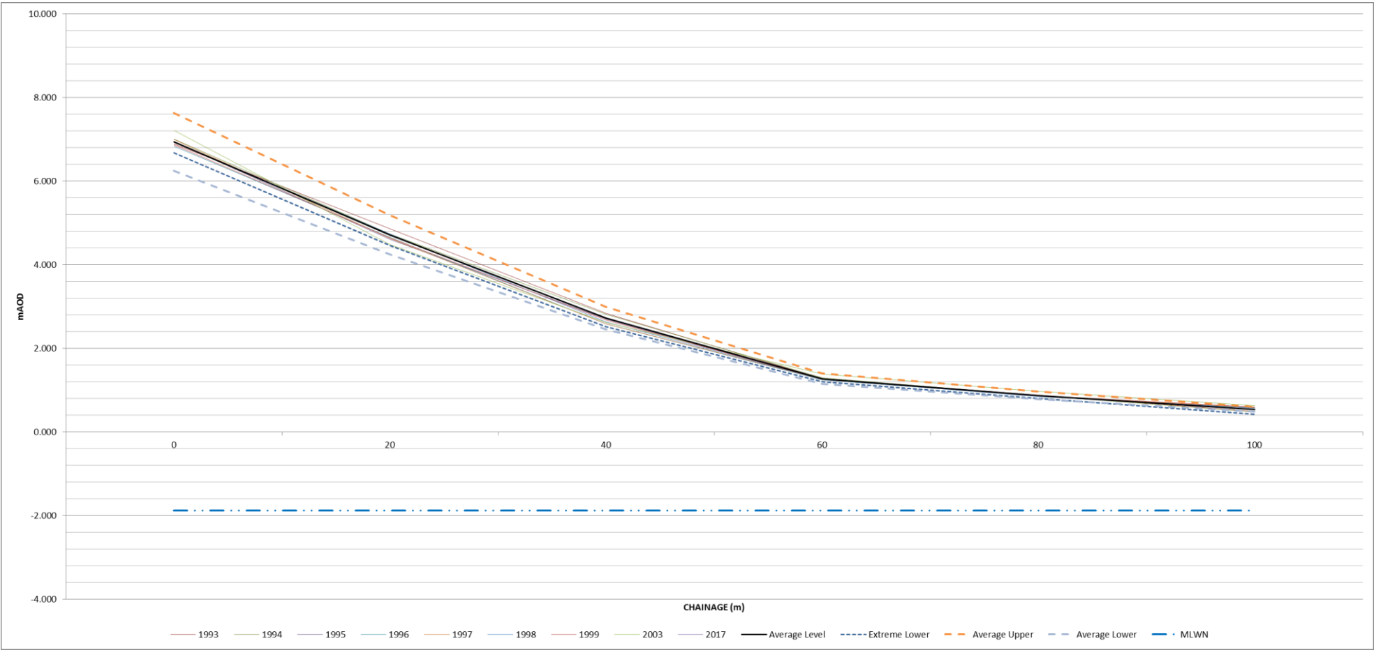
Figure I-66: Annual change of historic beach profiles, compared with extreme averages – HR19
