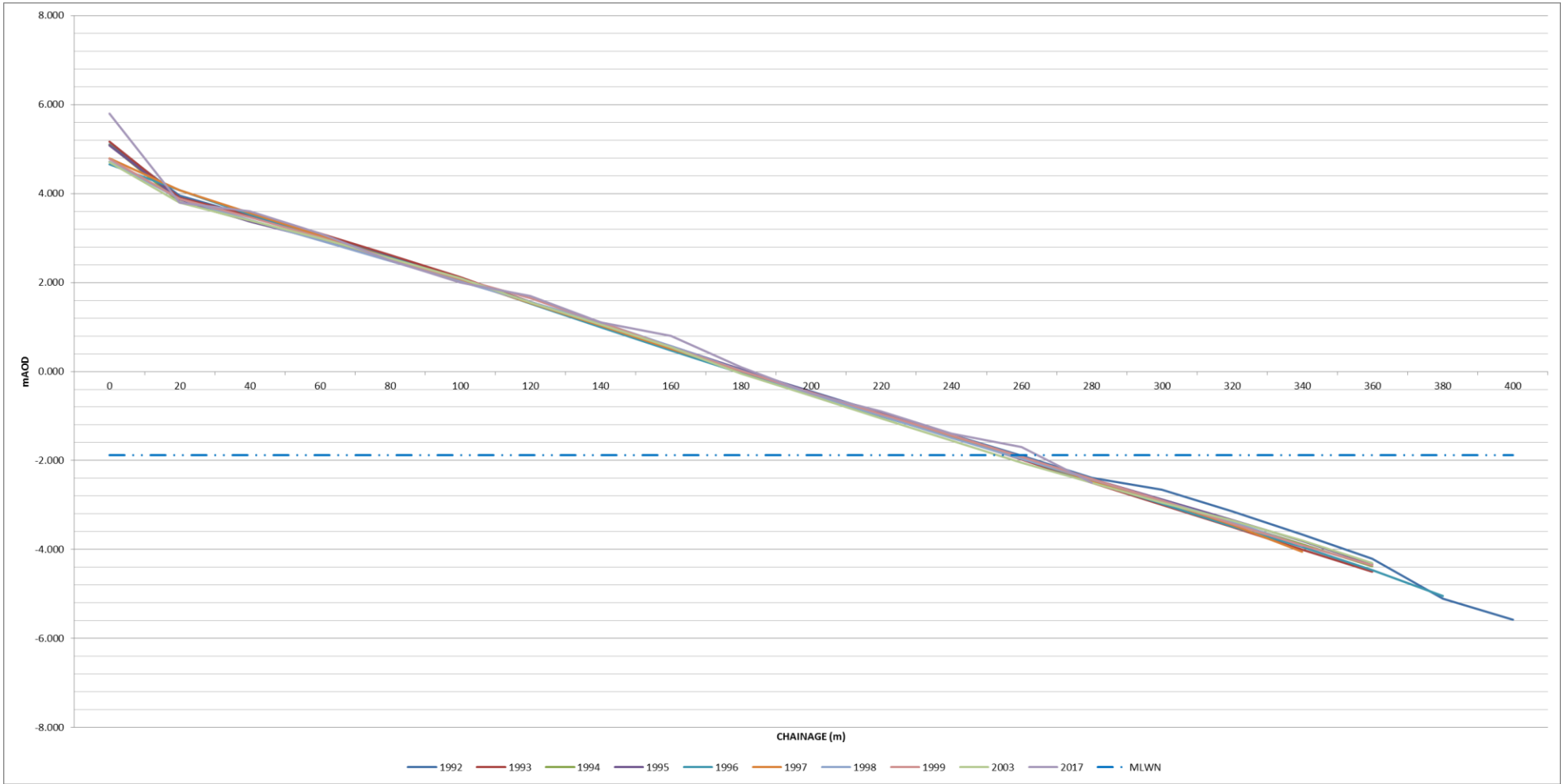
Figure I-25: Annual change of historic beach profiles – HR9
