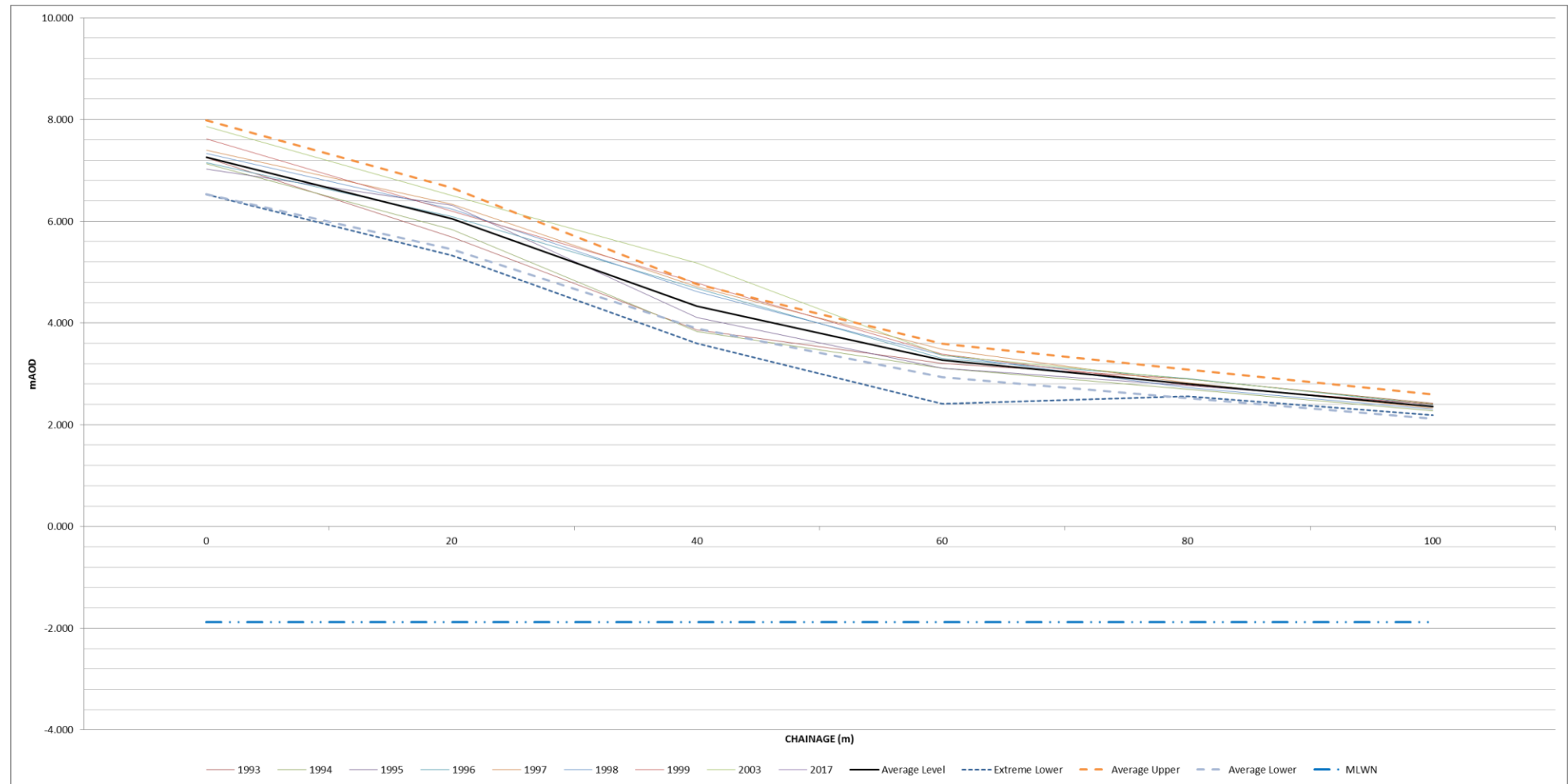
Figure I-64: Annual change of historic beach profiles, compared with extreme averages – HR17
