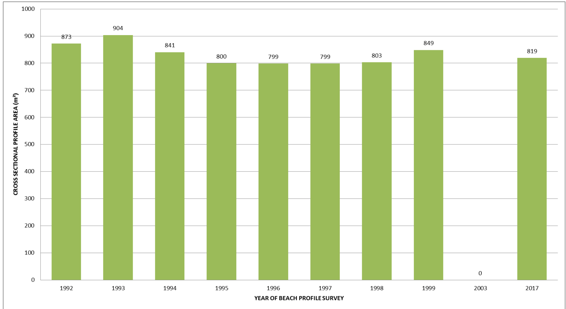
Figure I-73: Cross sectional Area of Annual Average Profiles – HR12
