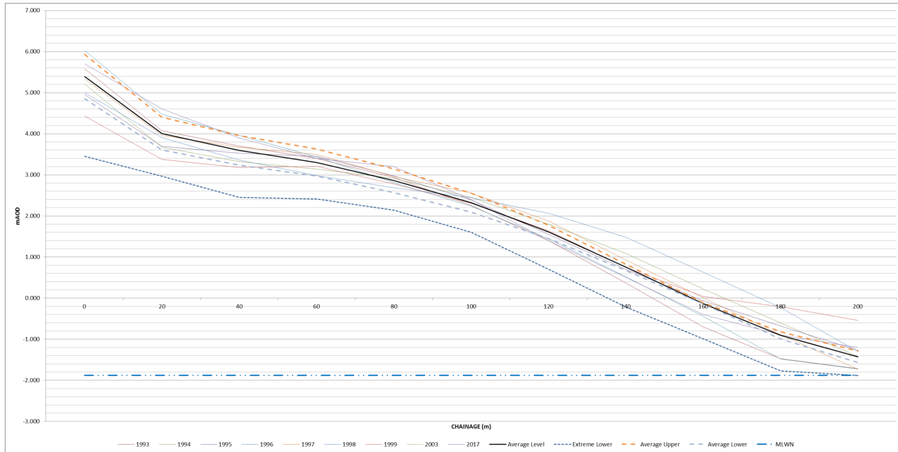
Figure I-49: Annual change of historic beach profiles, compared with extreme averages – HR2
