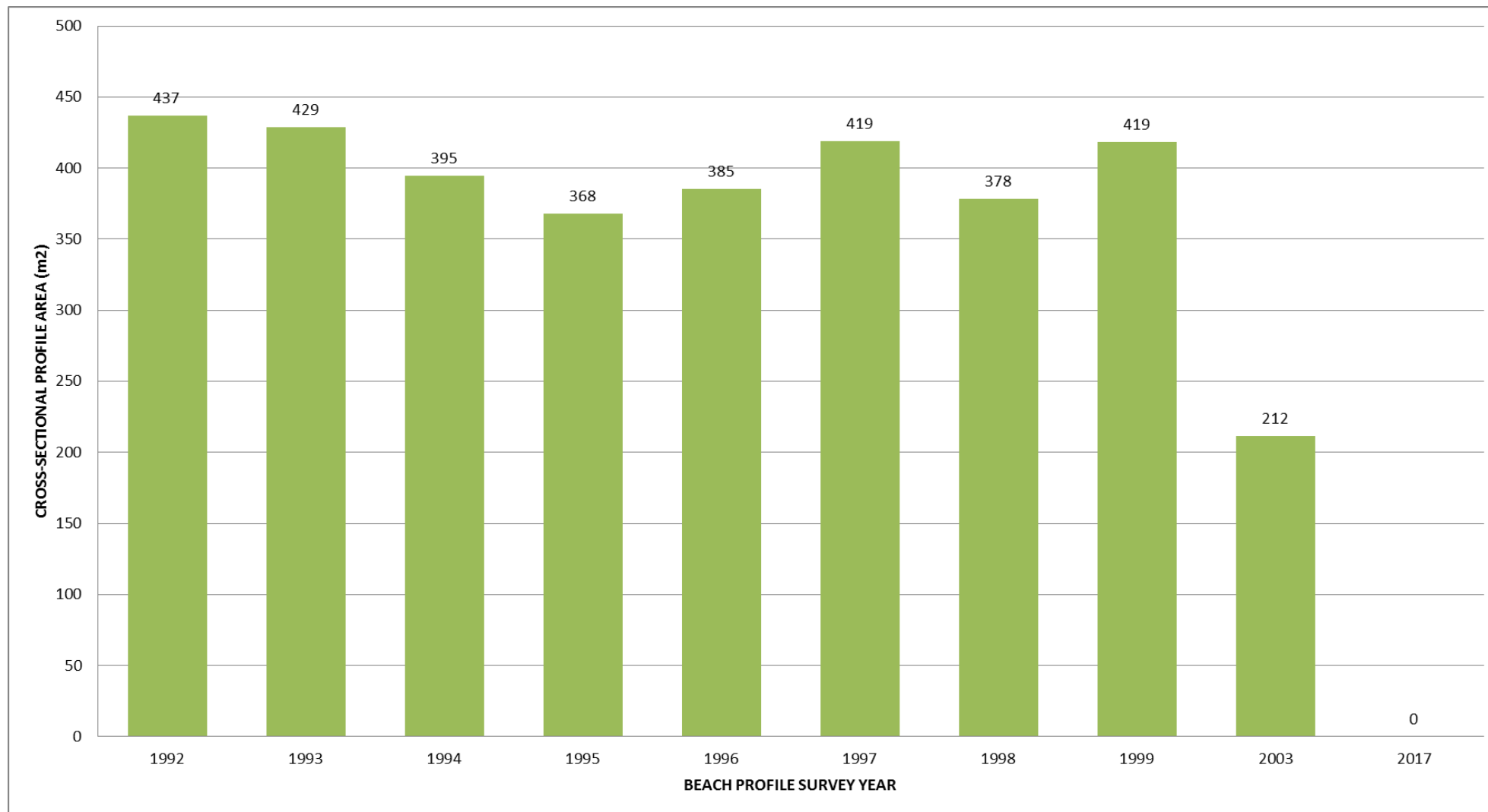
Figure I-74: Cross sectional Area of Annual Average Profiles – HR16
