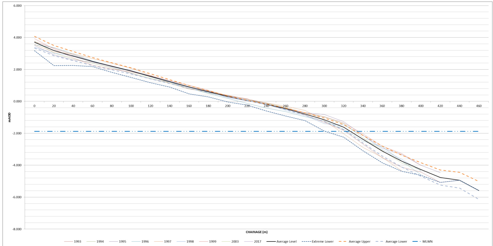
Figure I-50: Annual change of historic beach profiles, compared with extreme averages – HR3
