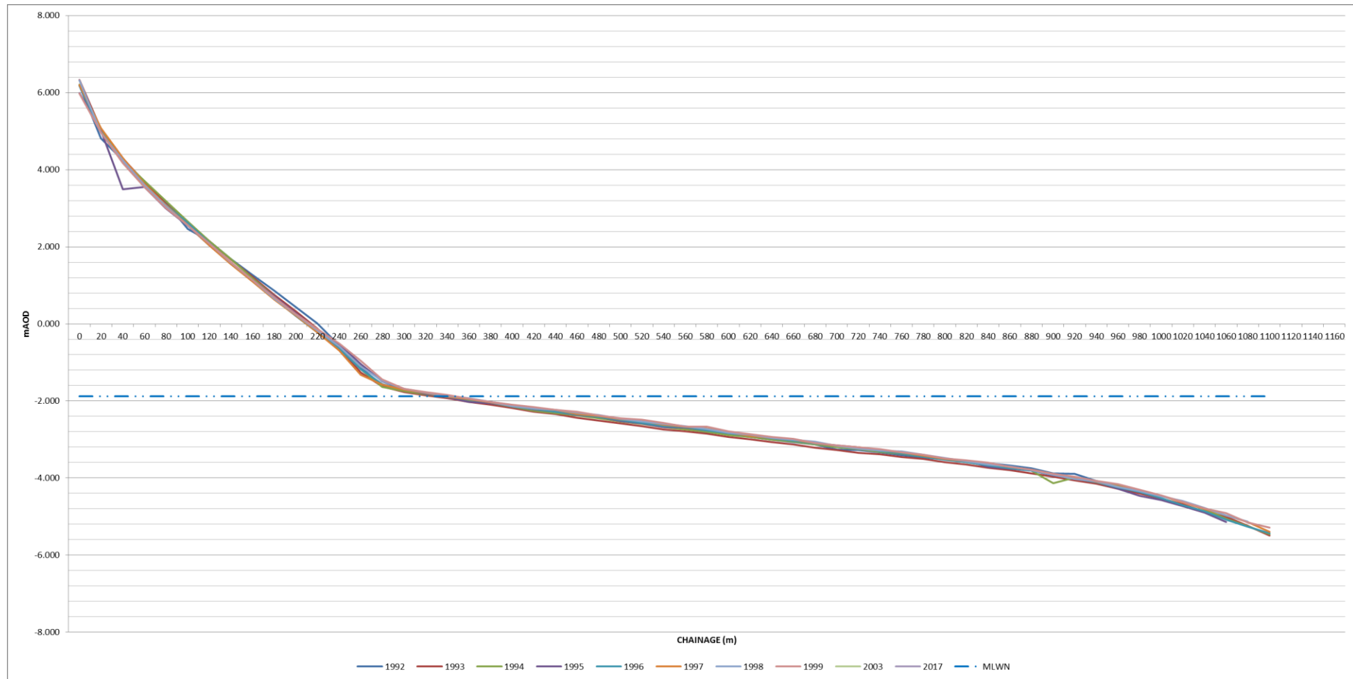
Figure I-29: Annual change of historic beach profiles – HR13
