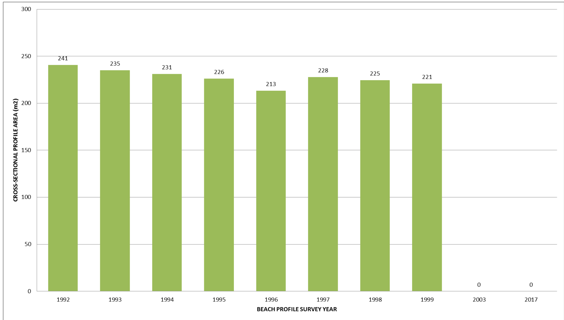
Figure I-71: Cross sectional Area of Annual Average Profiles – PSD8
