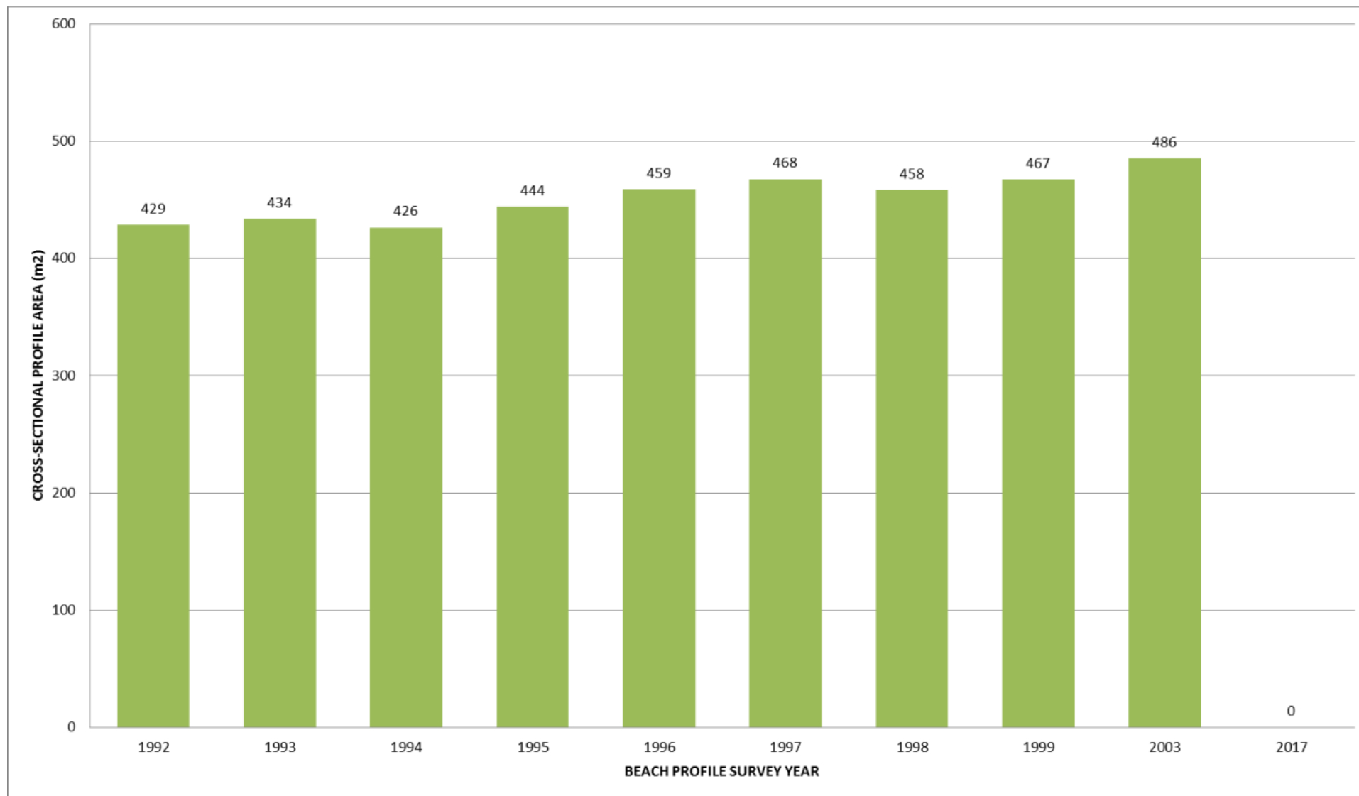
Figure I-75: Cross sectional Area of Annual Average Profiles – HR17
