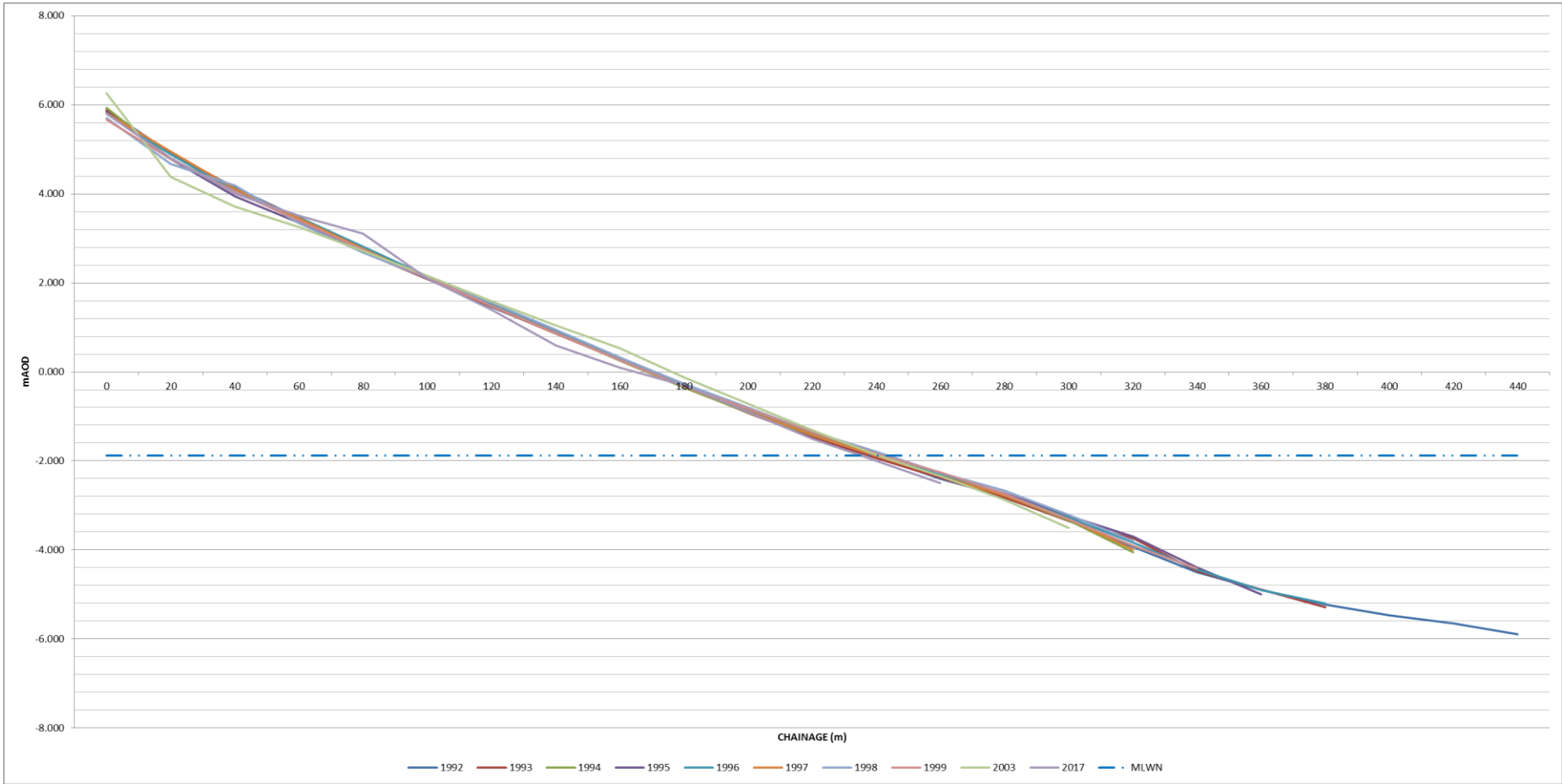
Figure I-24: Annual change of historic beach profiles – HR8
