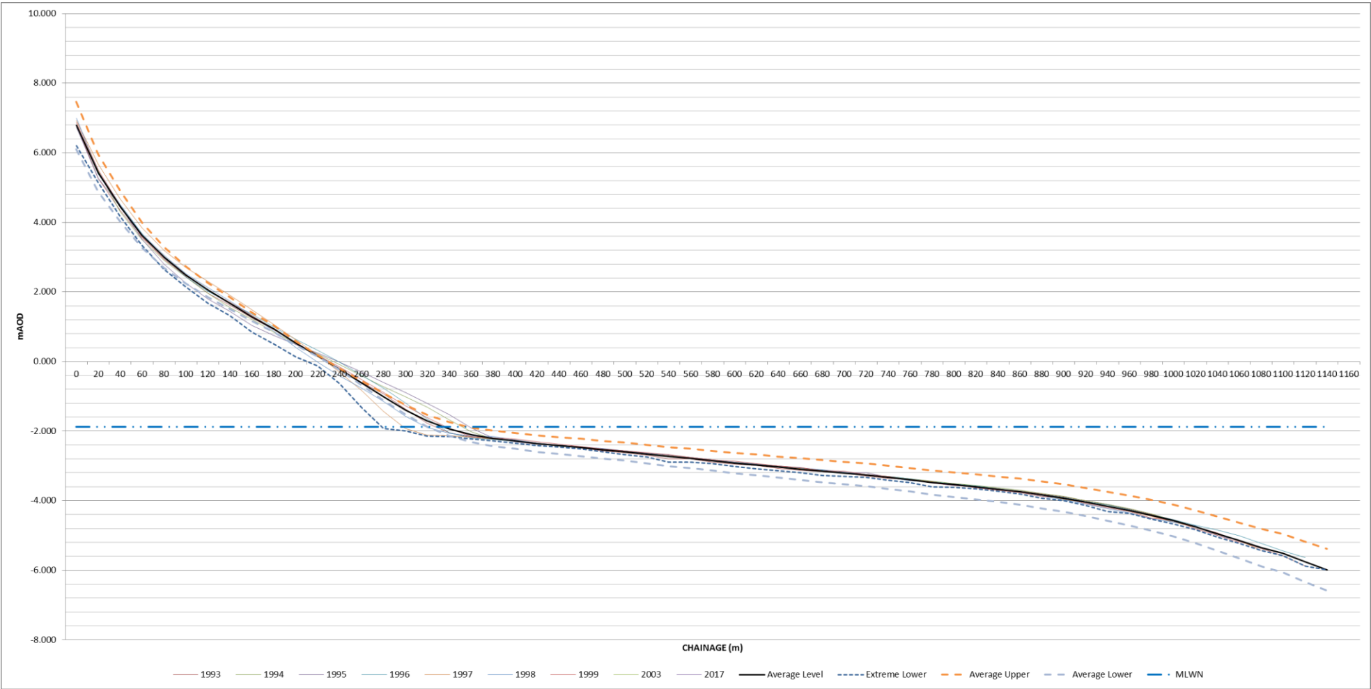
Figure I-61: Annual change of historic beach profiles, compared with extreme averages – HR14
