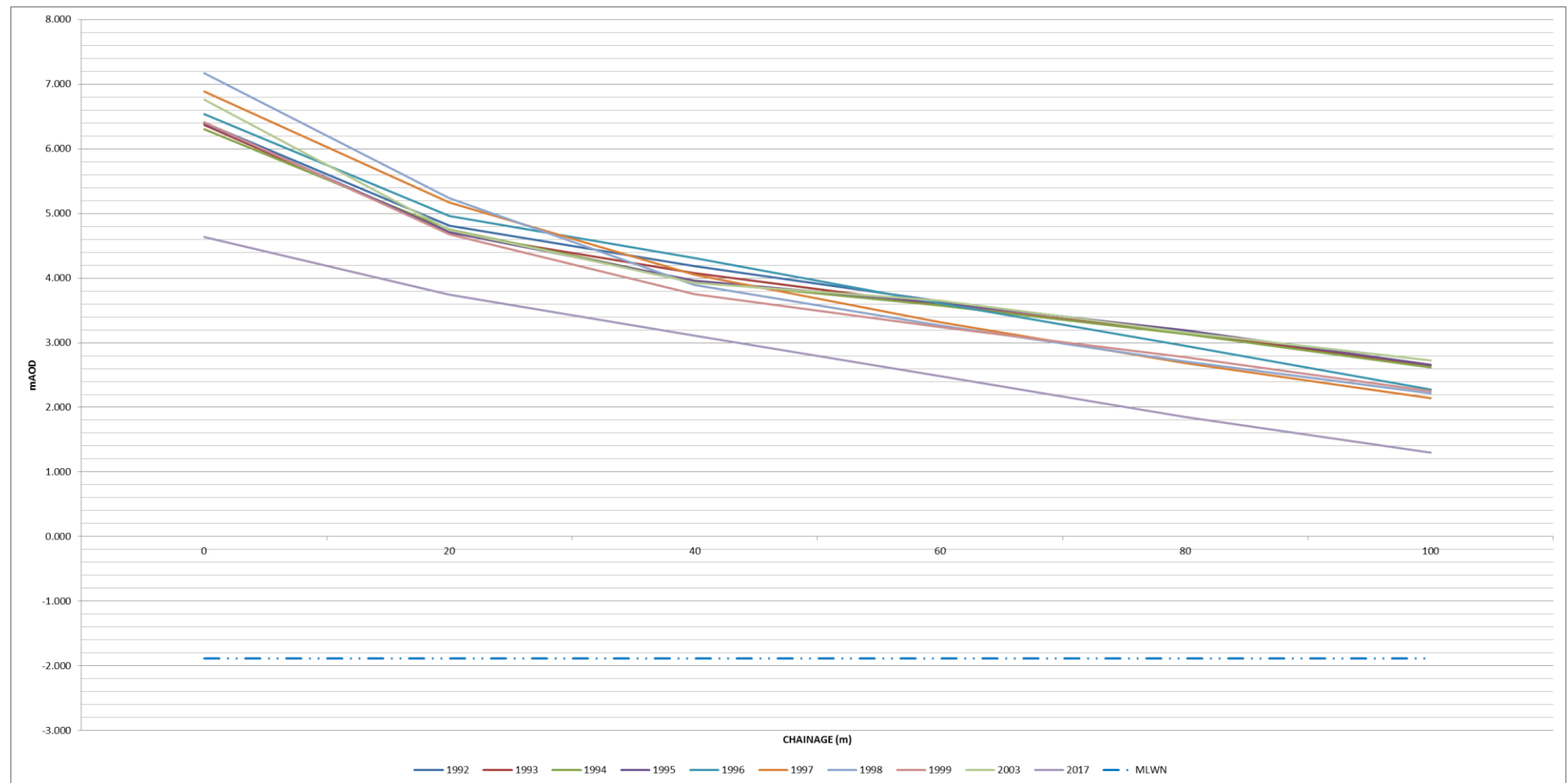
Figure I-34: Annual change of historic beach profiles – HR18
