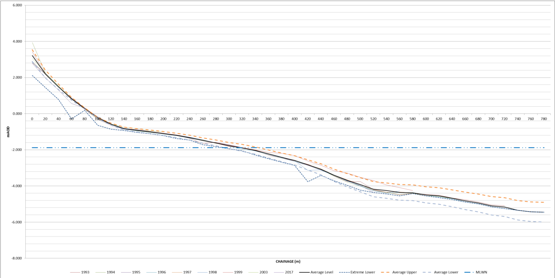
Figure I-63: Annual change of historic beach profiles, compared with extreme averages – HR16
