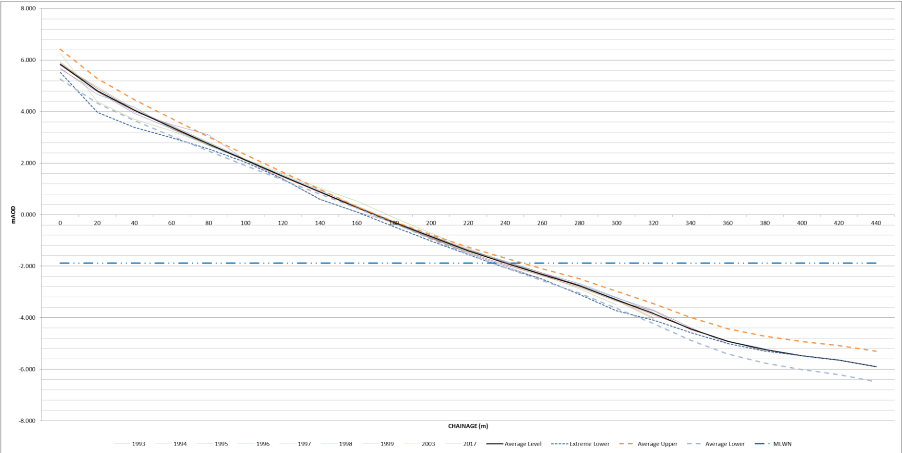
Figure I-55: Annual change of historic beach profiles, compared with extreme averages – HR8
