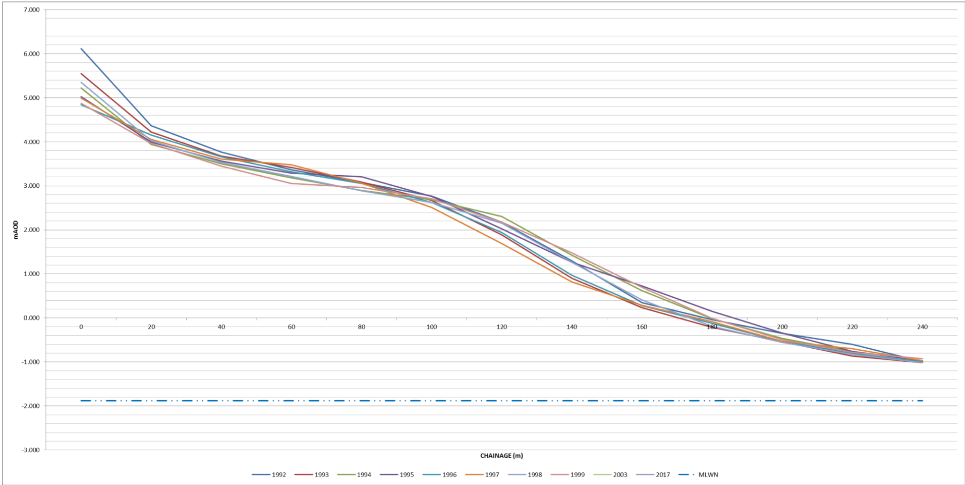
Figure I-17: Annual change of historic beach profiles – HR1
