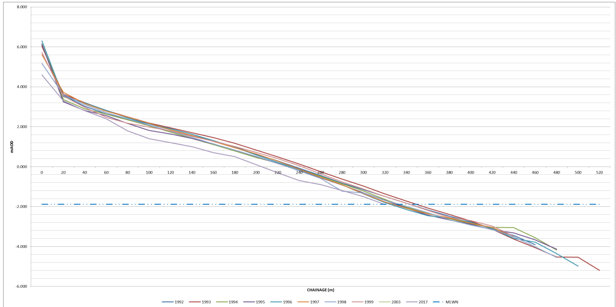
Figure I-22: Annual change of historic beach profiles – HR6
