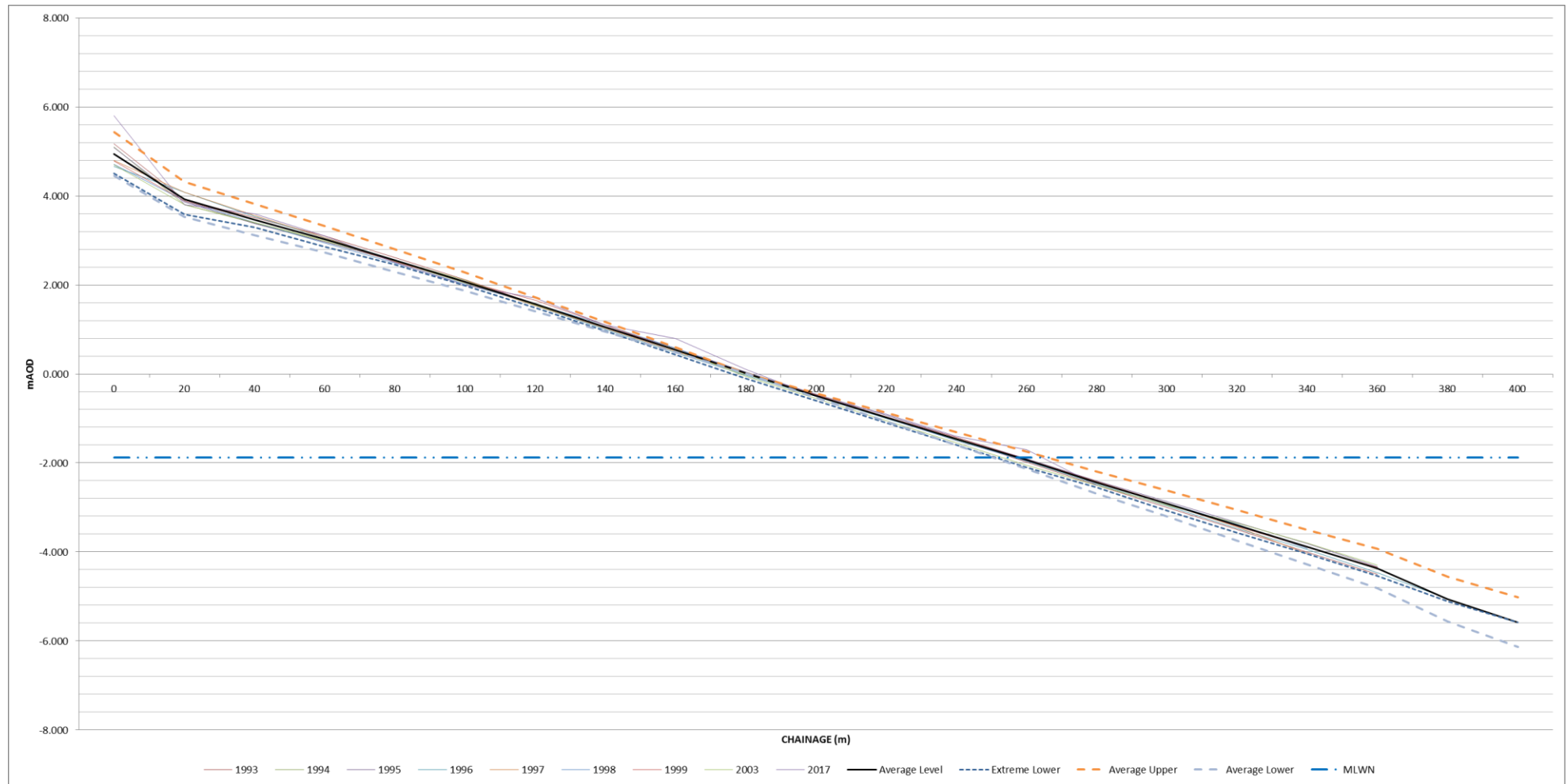
Figure I-56: Annual change of historic beach profiles, compared with extreme averages – HR9
