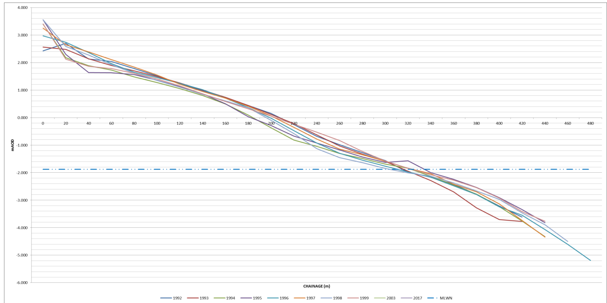
Figure I-21: Annual change of historic beach profiles – HR5
