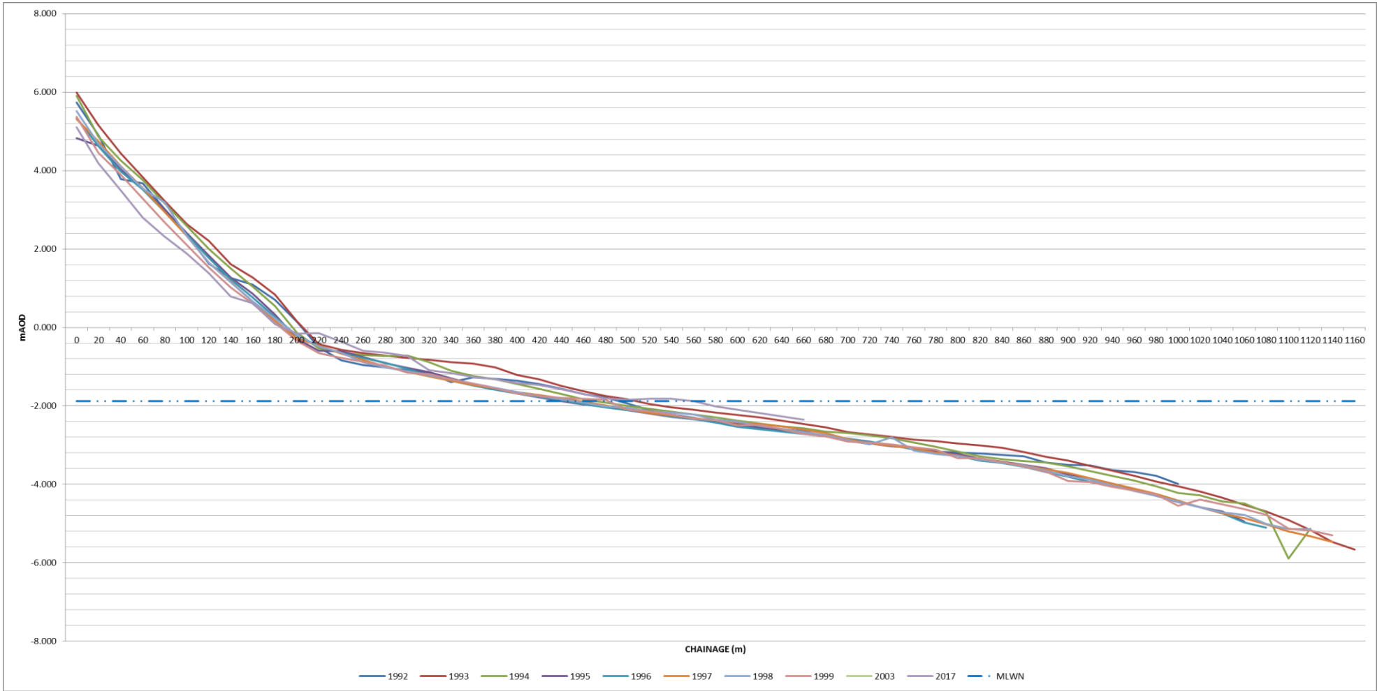
Figure I-28: Annual change of historic beach profiles – HR12
