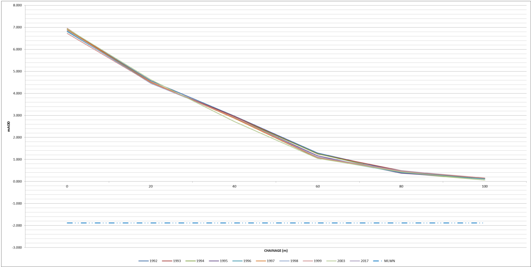
Figure I-38: Annual change of historic beach profiles – HR22
