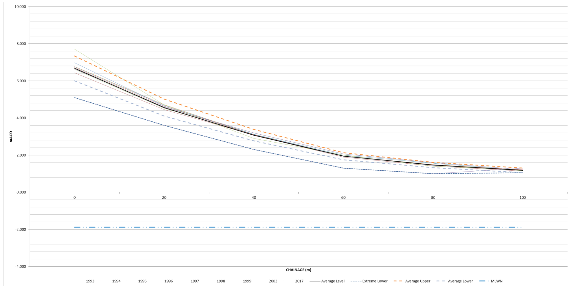
Figure I-68: Annual change of historic beach profiles, compared with extreme averages – HR21
