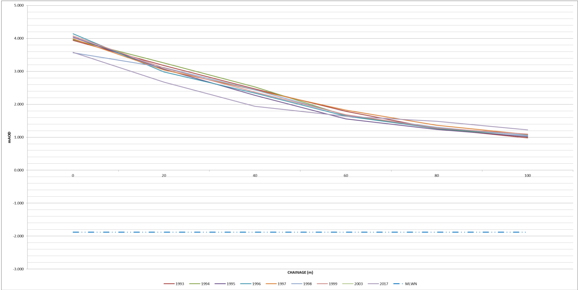
Figure I-8: Annual change of historic beach profiles – PSD1
