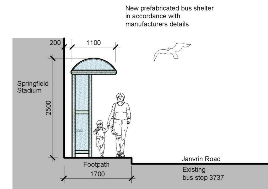
South Elevation
