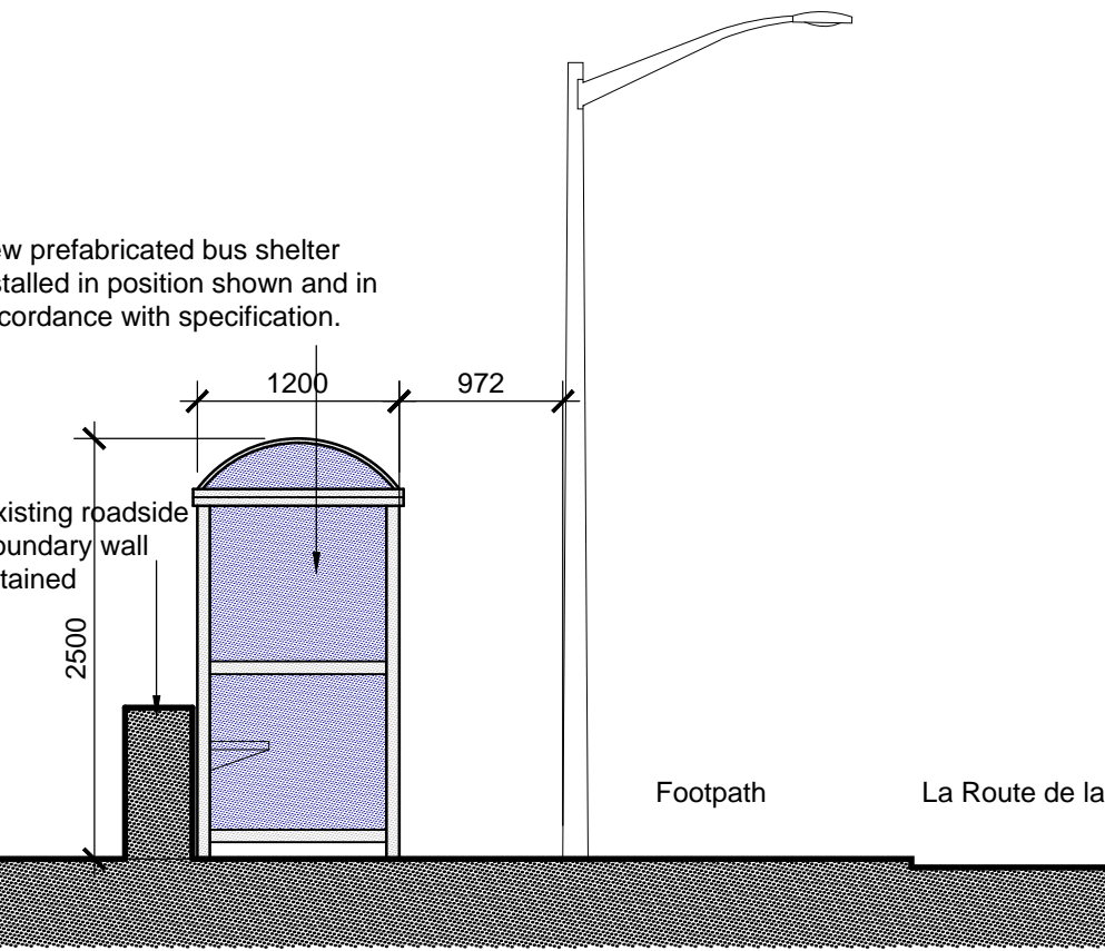
West Elevation
