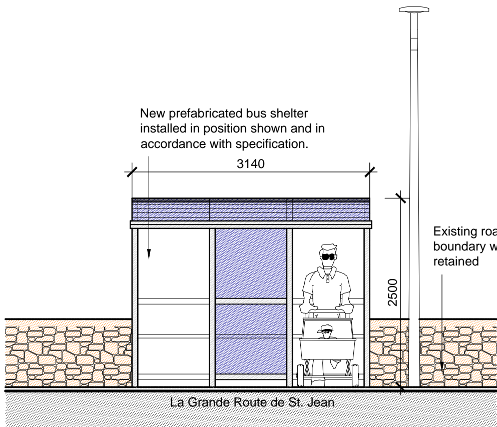
South Elevation
