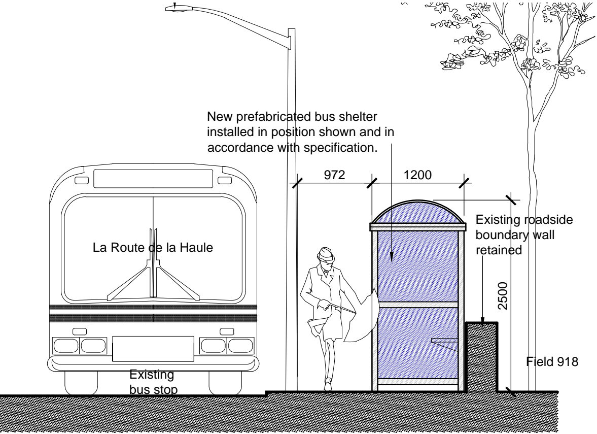
East Elevation
