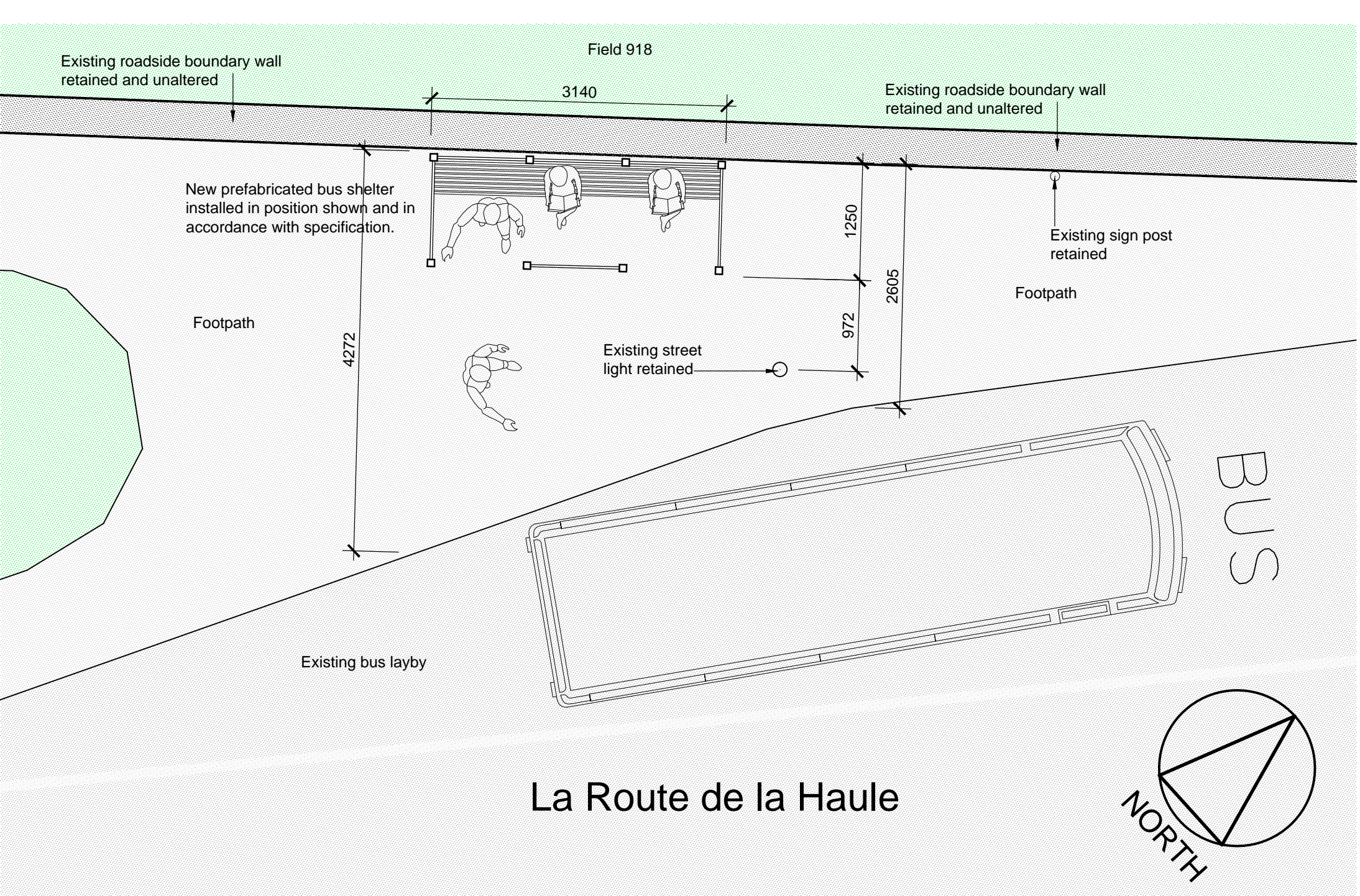
Plan
