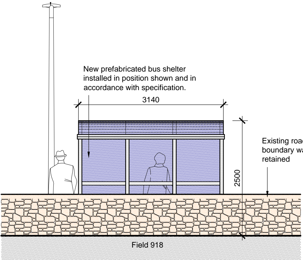
North Elevation
