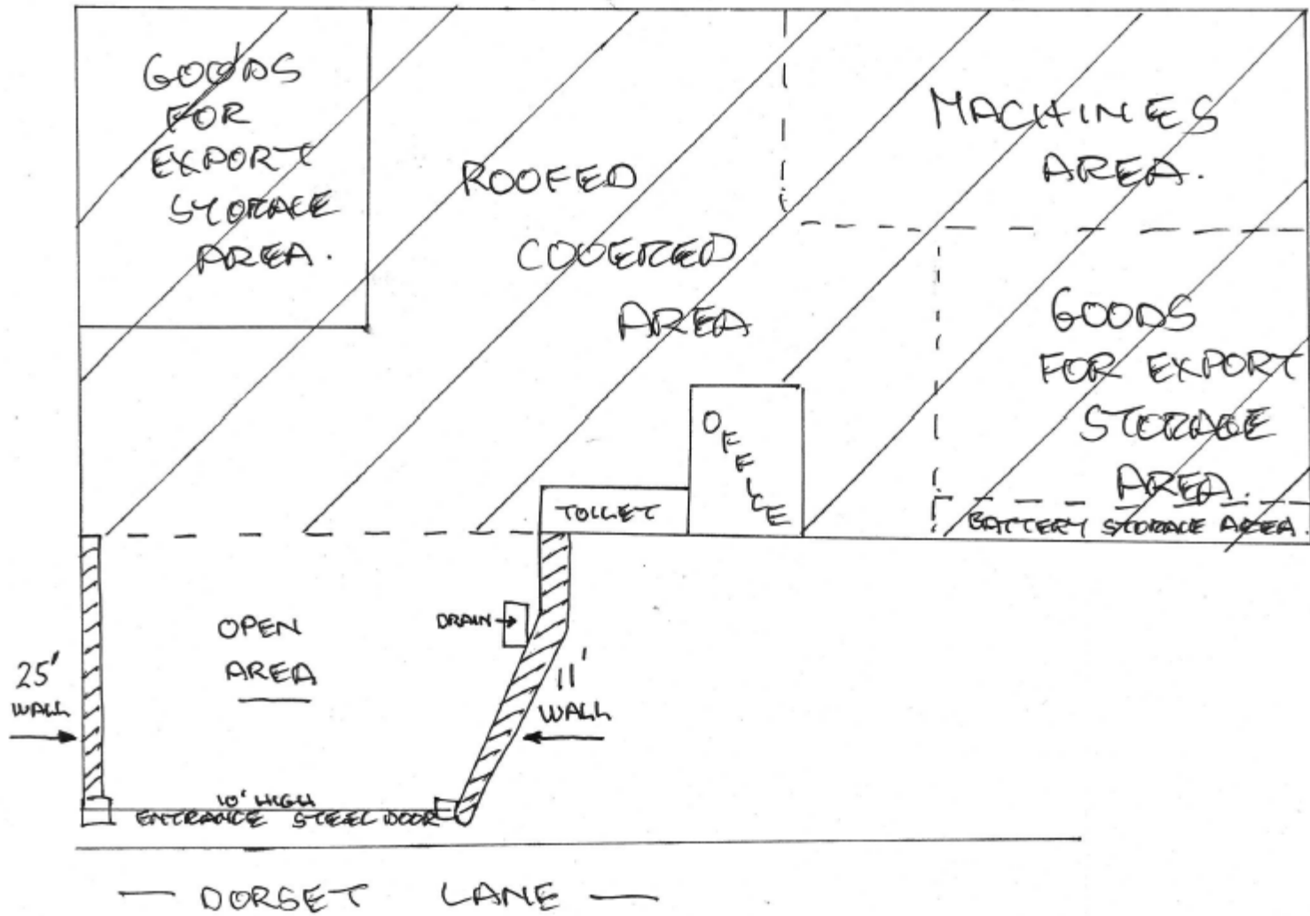
REvised SITE PLAN OF ATLAS WORKS (NOT TO SCALE) 2/1/61/3
