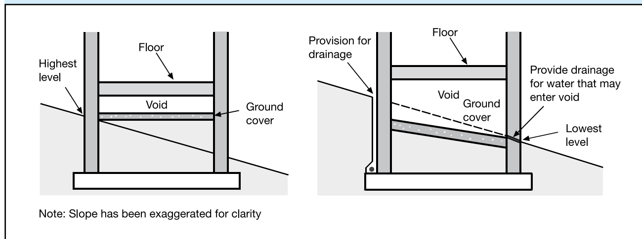
Diagram 5 Suspended floor – preventing water collection (see paragraph 4.14(a)(ii))
