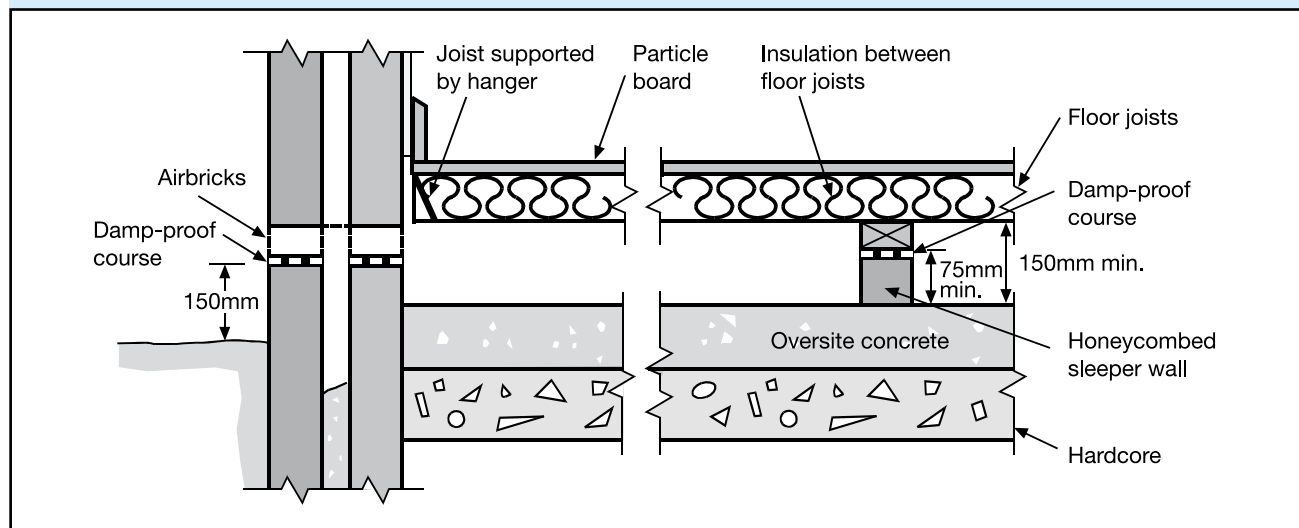
Diagram 4 Suspended timber floor – construction (see paragraph 4.14(a)(i))
