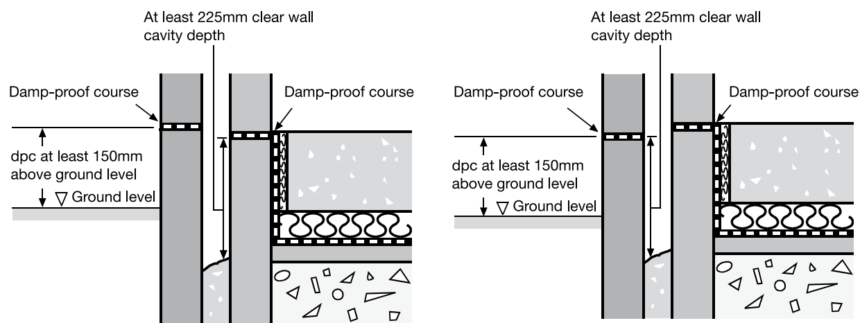
Diagram 8 Protecting inner leaf (see paragraph 5.5(c))
