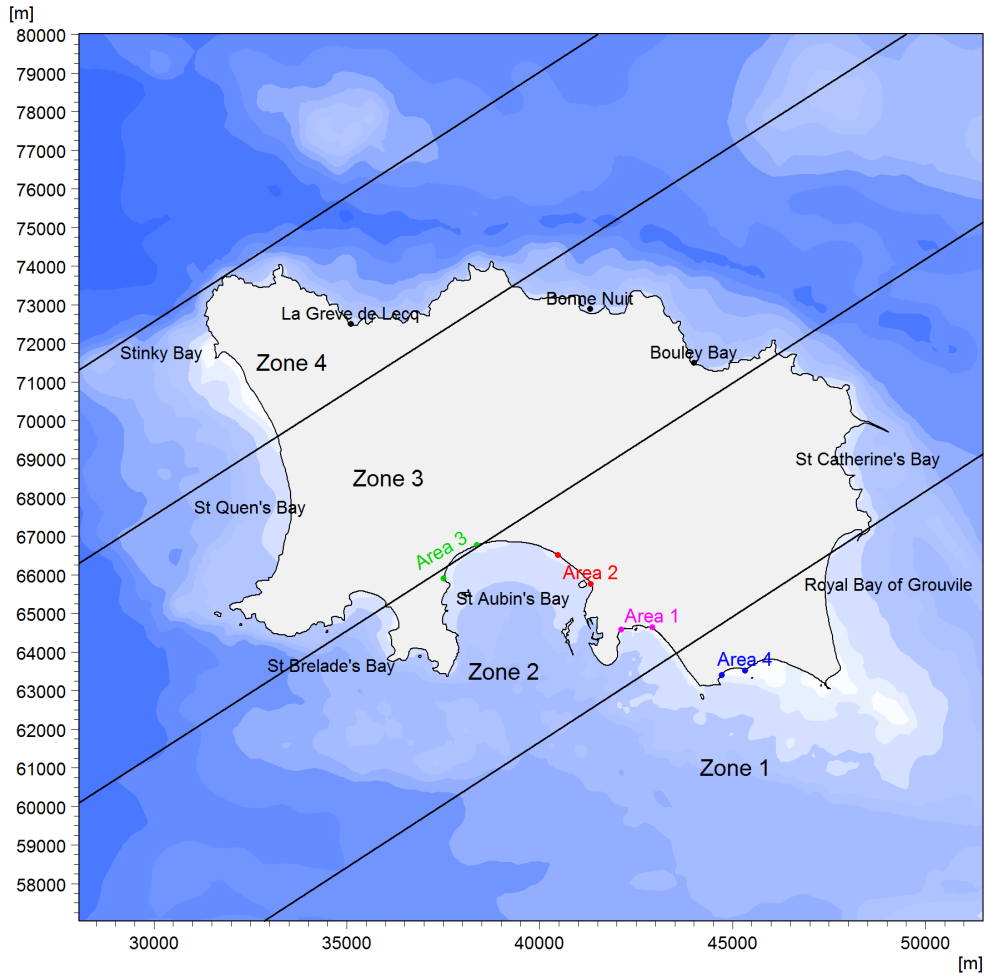
Figure B-3: Zones Defined for Still Water Level Adjustments
